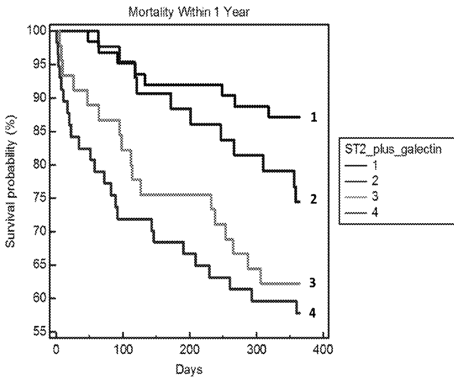
Figure 3: K-M Analysis of ST2 plus Galectin-3
