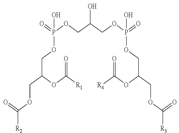
Cardiolipin
