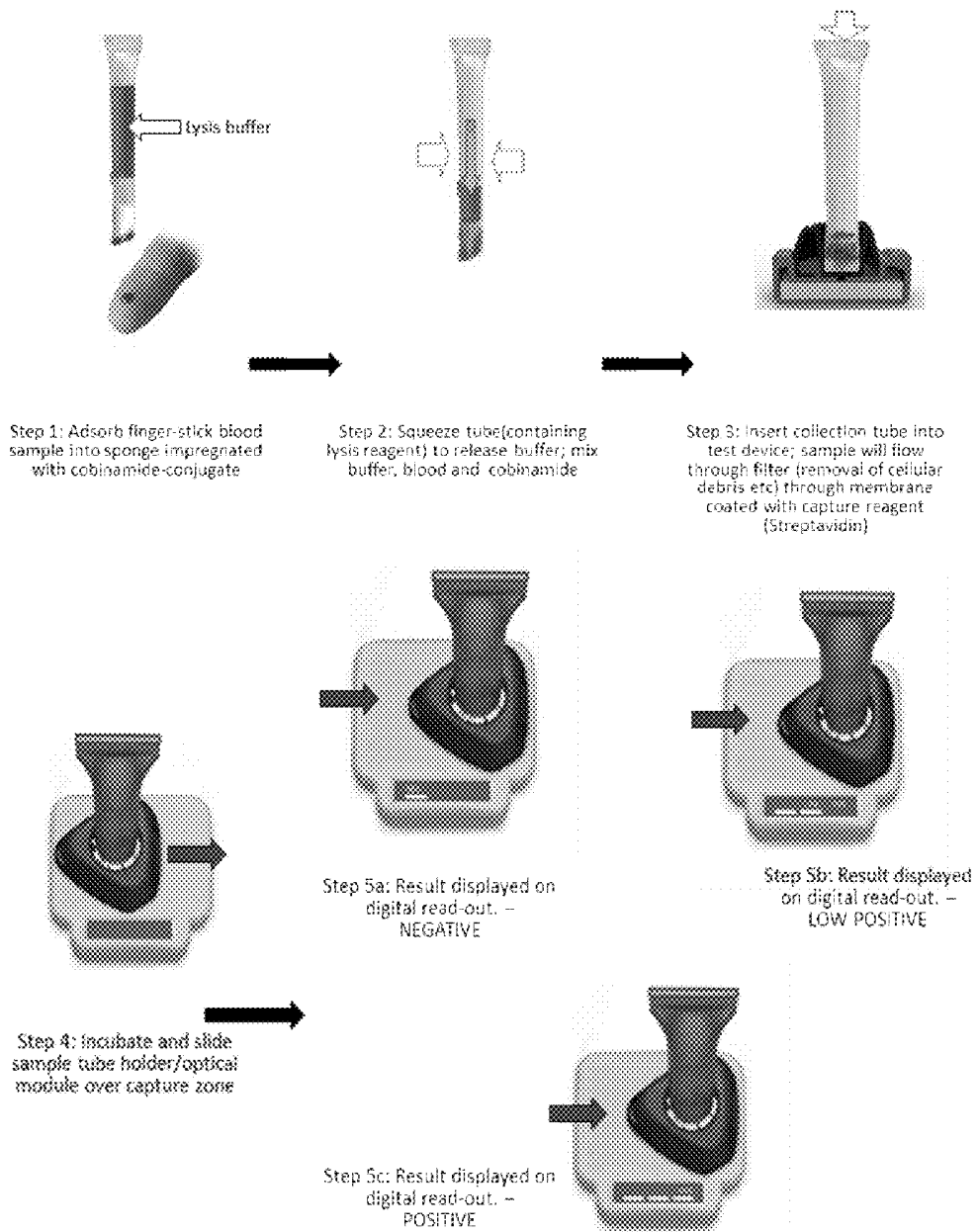
Figure 10 Concept of field-deployable, rapid cyanide test
