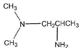
1-dimethylamino-2-propylamine
