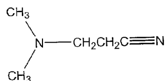
3-dimethylaminopropionitrile
