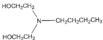
N-butyl-diethanolamine
