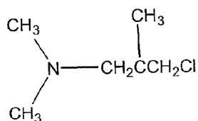
3-dimethylamino-2-methylpropyl chloride
