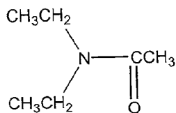
N,N-diethylacetamide
