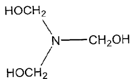
trimethanolamine
