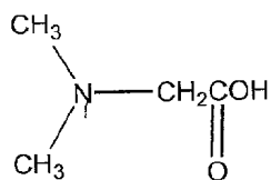
N,N-dimethylglycine
