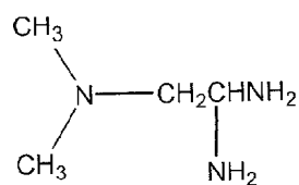
N,N-dimethylguanidine
