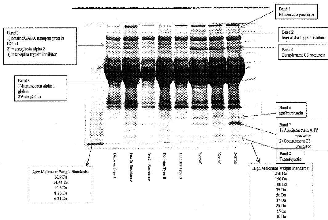
HiQ 1-(Elution) Insulin Resistance vs. Normal FIGURE 1
