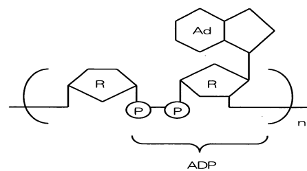
Structural formula of ADPR
