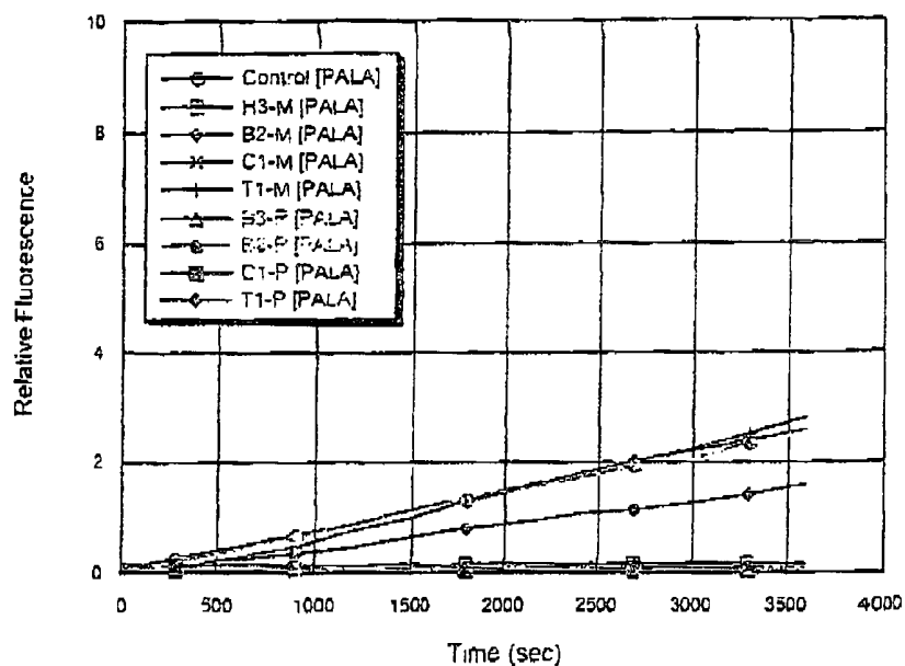
Figure 6. Assay for mold using peptide pala. Legend abbreviations: H3 = Cladosporium (house mold), B2 = Penicillium (bread mold), C1 = Cladosporium (cheese mold), T1 = Cladosporium (tomato mold), B3 = Mucor (bread mold), M = malt media, P = potato dextrose media.
