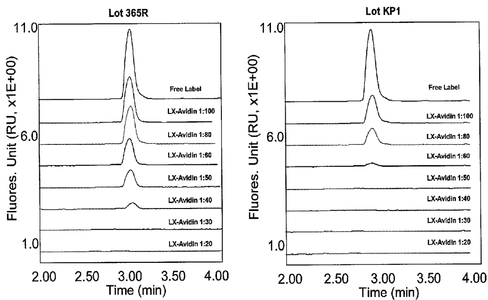
Figure 3. Quantitation and comparison of two latex-avidin lots by CE-LIF: latex-avidin A/C ratio 0.15; latex-avidin lots, 365R and KP1; latex-avidin dilutions, 1:20 to 1:100; biotin-fluorescein 3.68 \times 10^{-8} M.
