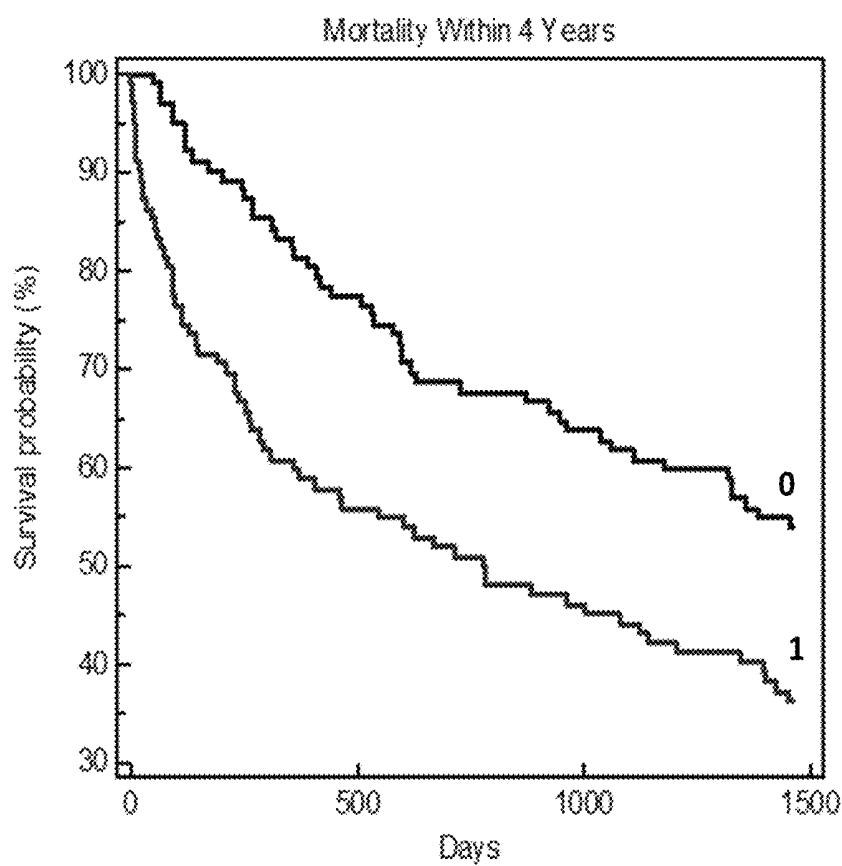
Figure 2B: ST2 K-M Analysis for 4 years (log rank p=0.0022 )
