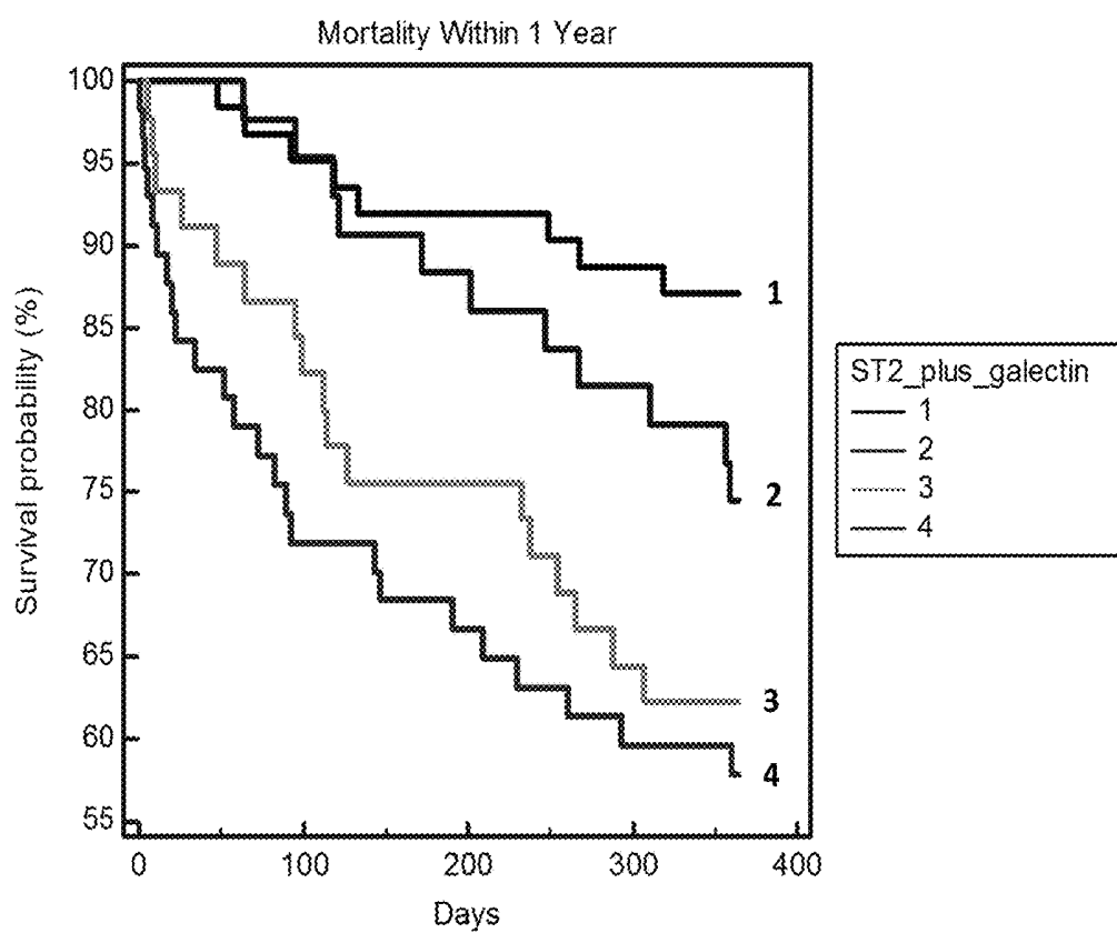
Figure 3: K-M Analysis of ST2 plus Galectin-3
