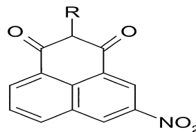
Basic Structure of N- (Aryl Substituted) - naphthalidimides
