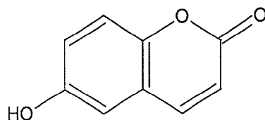
7-Hydroxycoumarin
