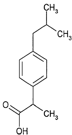
(s) -Ibuprofen
