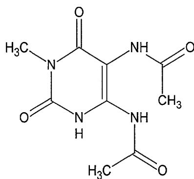
AFMU (5-acetamido-6-formylamino-methyluracil)
