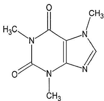
Caffeine (1,3,7-trimethylxanthine)
