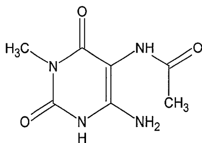
AAMU (5-acetamido-6-amino-methyluracil)
