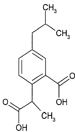
2-carboxvibuprofen
