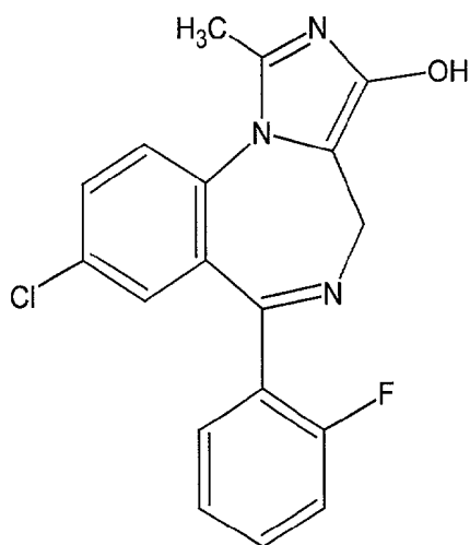
1-OH-MDZ (1-Hydroxymidazolam)
