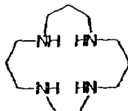
1,4,8,12-tetraaza cyclopentadecane
