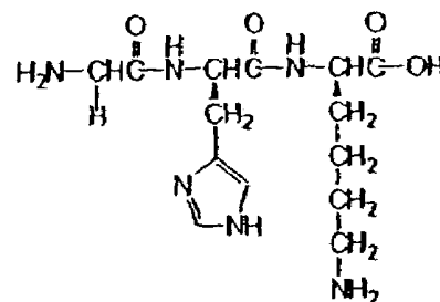
Glycyl-histidyl-lysine (GHK)
