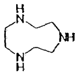
1,4,7-Triazacyclononane
