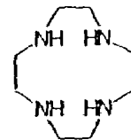
1,4,7,10-Tetraaza cyclo dodecane
