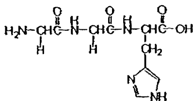
Glycyl-glycyl-histidine (GGH)
