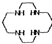
1,4,8,11-Tetraaza cyclotetradecane
