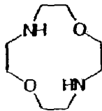
1,7-Dioxo-4,10-diazacyclododecane
