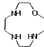
1-Oxa-4,7,10-triazacyclododecane
