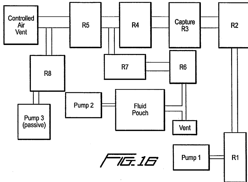
Fluidic Schematic for i-STAT immunocarbidge
