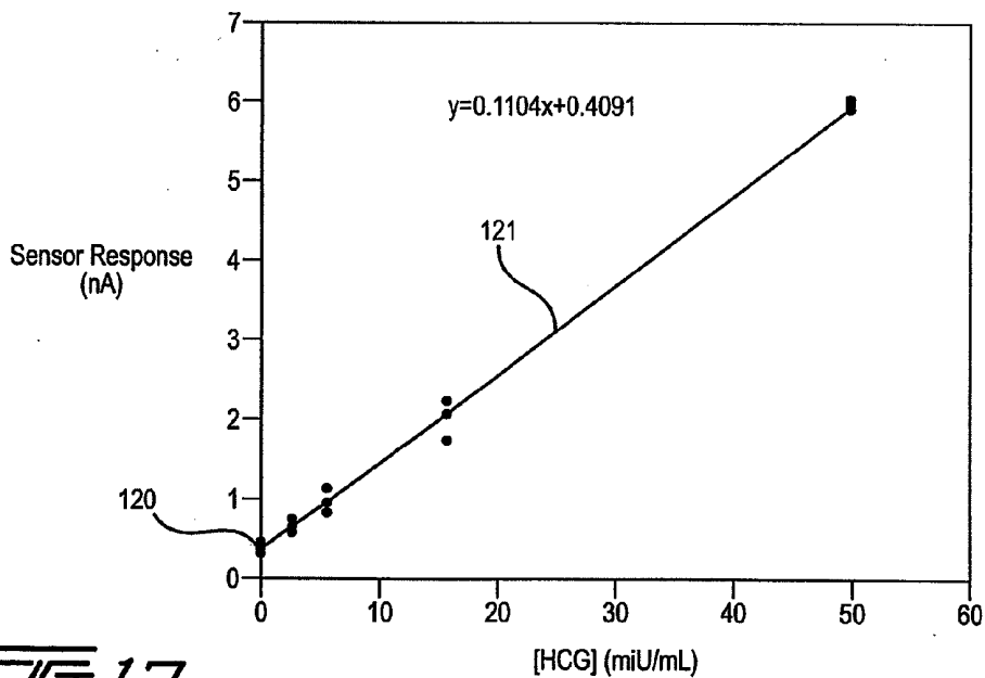
Sensor Response vs [HCG]
