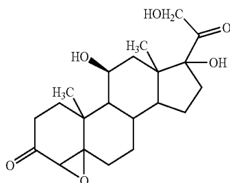
Cortisol Epoxide
