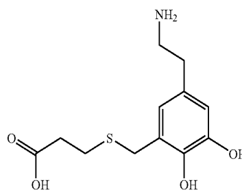
Dopamine acid
