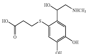
Epinephrine acid
