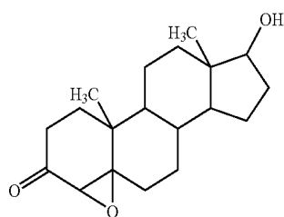
Testosterone Epoxide
