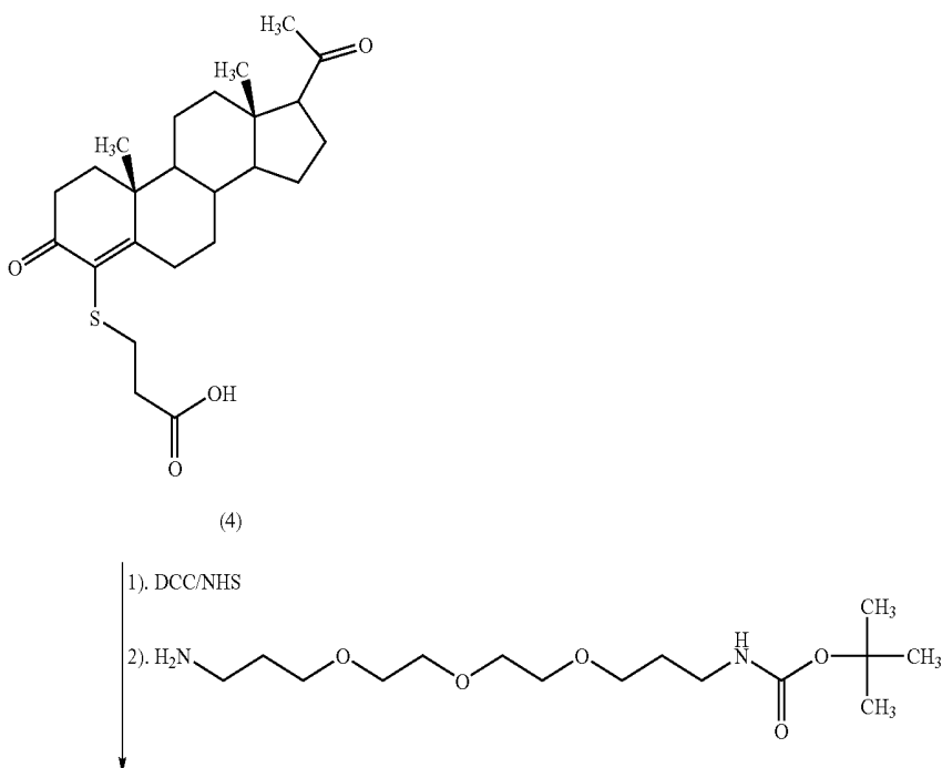
Reaction Scheme 2
