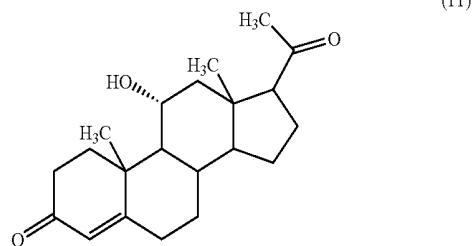
11 \alpha -Hydroxyprogesterone
