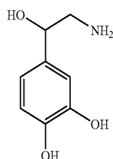
nor-Epinephrine
