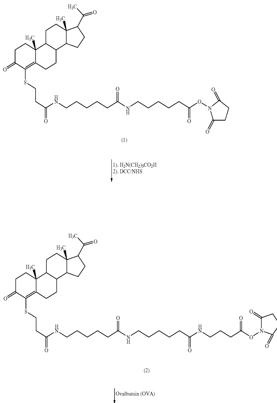
Reaction Scheme 1
