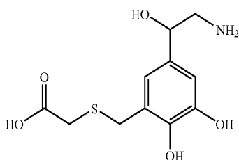
nor-Epinephrine acid
