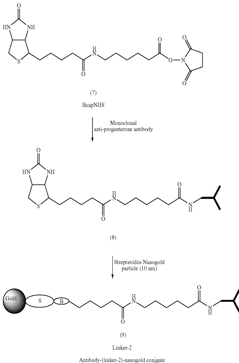
Reaction Scheme 3
