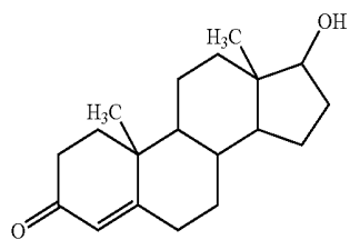
Testosterone
