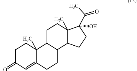
17 \alpha -Hydroxyprogesterone
