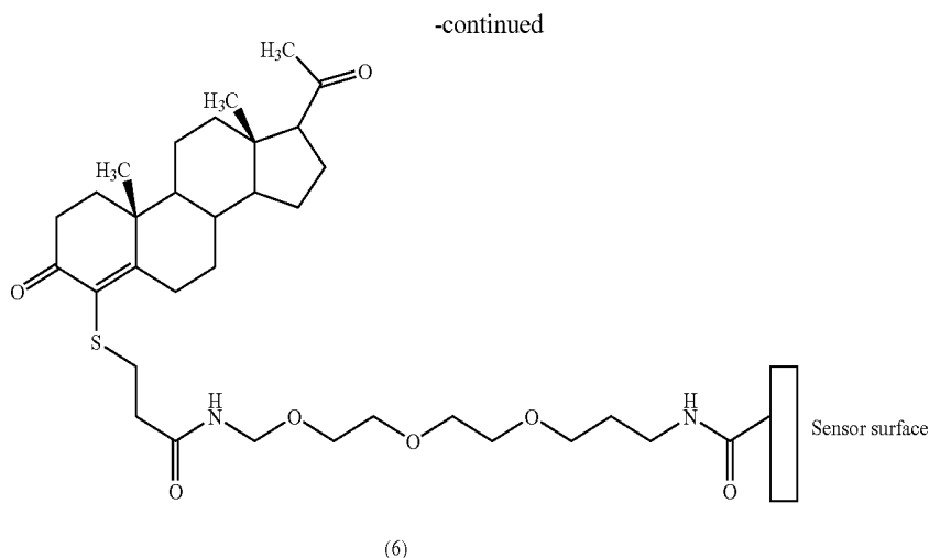
Synthesis of a progesterone-PEG (linker-1) derivative and its in-situ immobilization onto a sensor surface
