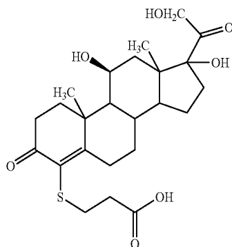
Cortisol Epoxide
