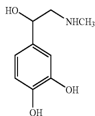
Epinephrine
