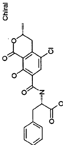
Ochratoxin A
