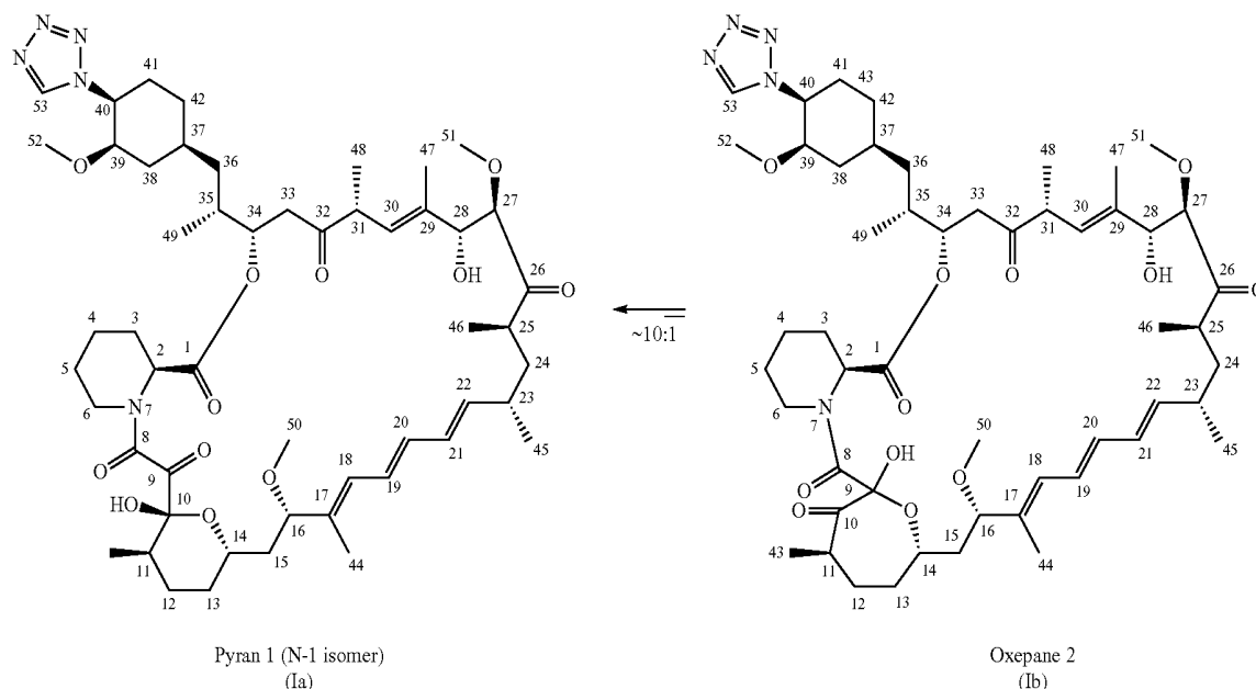
Formula D. The isomers of zotanolimus
