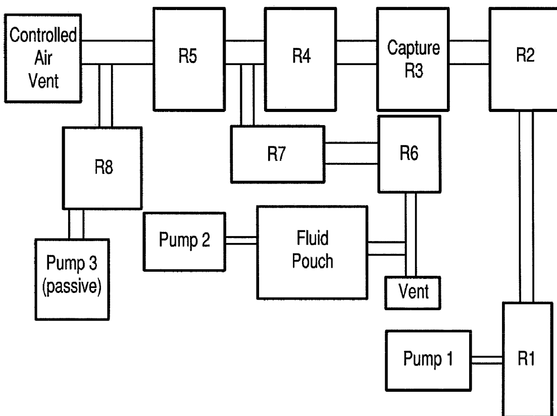
Fluidic Schematic for i-STAT immunocartridge
