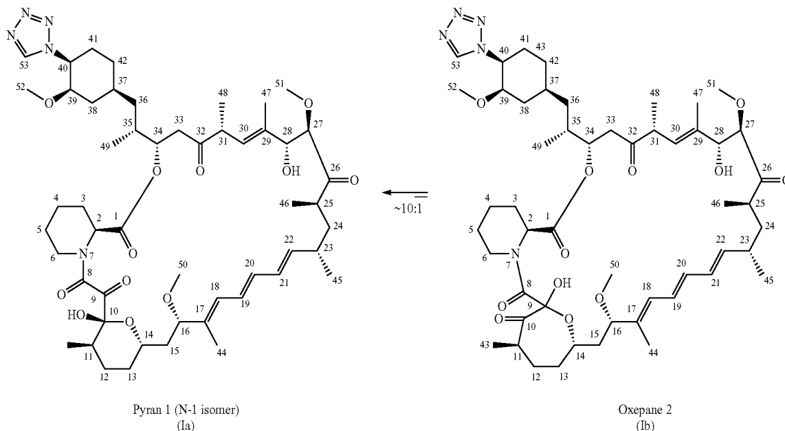
Formula D. The isomers of zotarolimus
