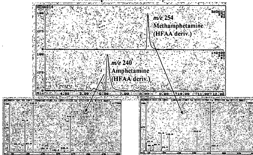
Figure 2: On-Line HFAA Derivatization/SFE of Amphetamine and Methamphetamine from Spiked Hair
