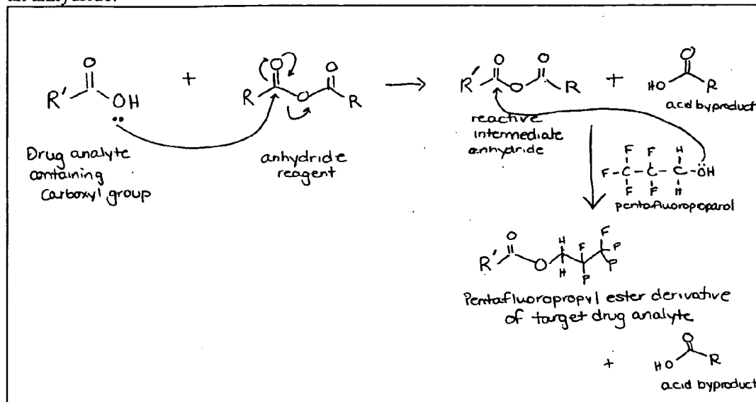
Figure 3: Esterification of a carboxyl group using pentafluoropropanol in the presence of an anhydride.
