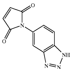
Benzotriazole Maleimide
