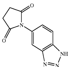
Benzotriazole Succinimide
