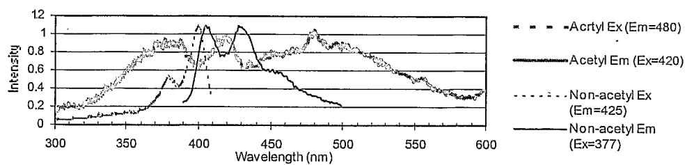
FIGURE 20 Fluorescent Property of Acetylated and Non-acetylated Anthracene Sensor
