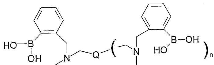
FIGURE 1A: Shinkai Dye Q is a fluorophore; n = 0 or 1
