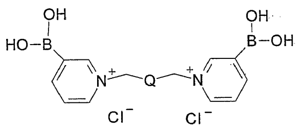
FIGURE 1B: Norrild Dye Q is a fluorophore
