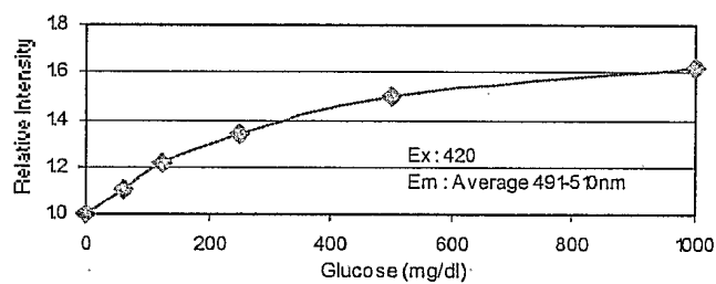
FIGURE 21 Glucose Response of Acetylated Anthracene Saccharide Sensor
