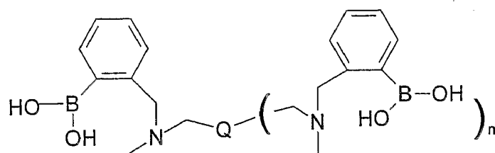
FIGURE 1A: Shinkai Dye Q is a fluorophore; n = 0 or 1
