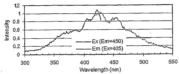
FIGURE 17 Fluorescent Property of Single-Arm Fluorophore Linked Sensor
