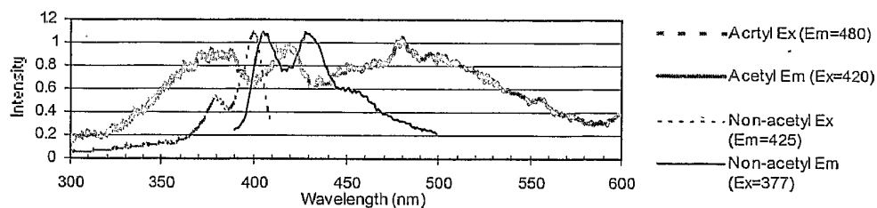
FIGURE 20 Fluorescent Property of Acetylated and Non-acetylated Anthracene Sensor
