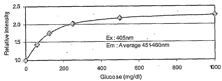
FIGURE 18 Glucose Response of Single-Arm Fluorophore Linked Sensor
