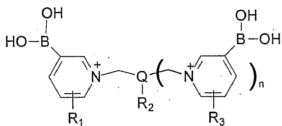
FIGURE 2B: Norrild Dye
