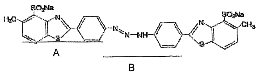
Thiazin yellow
