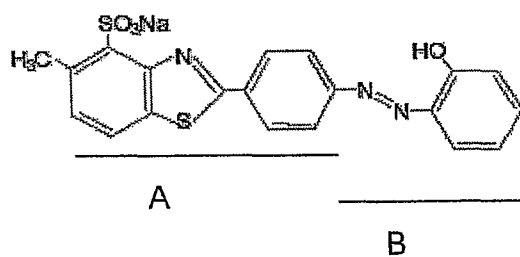
Benzothiazole analogue
