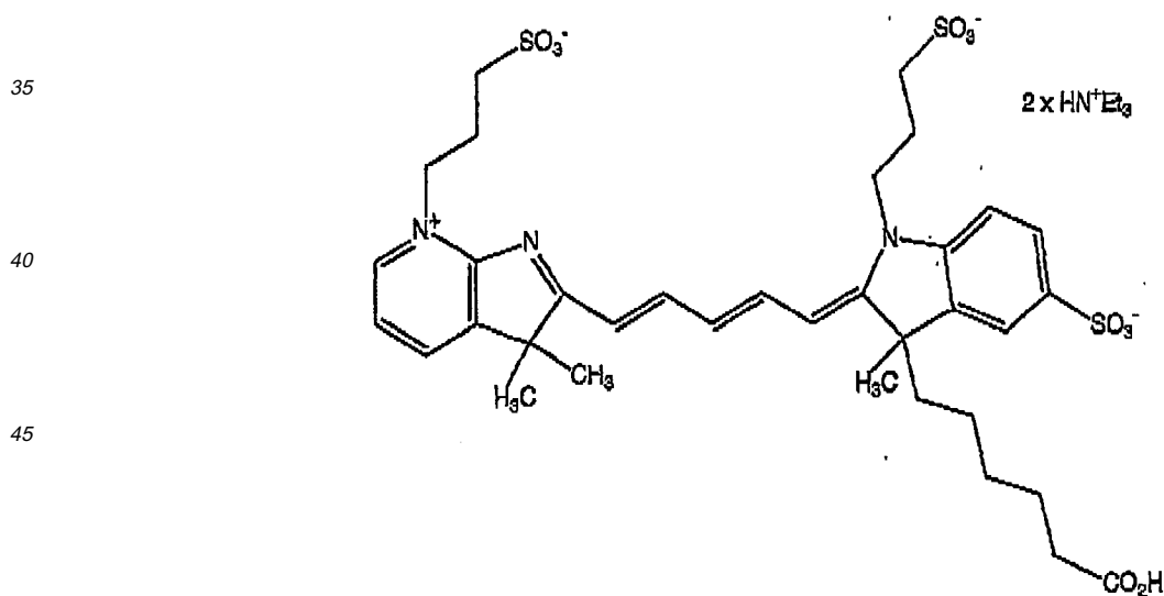
Compound 68
