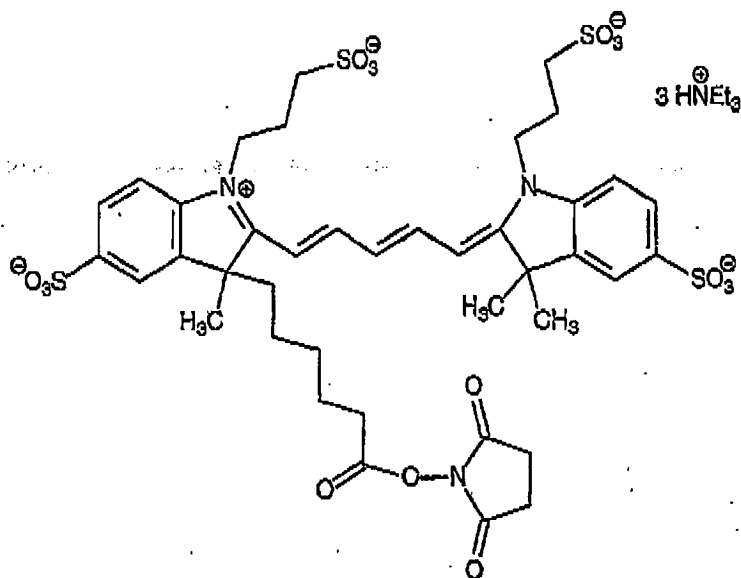
Compound 9
