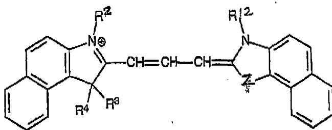
Formula XIV
