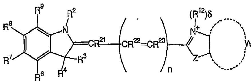
Formula XI
