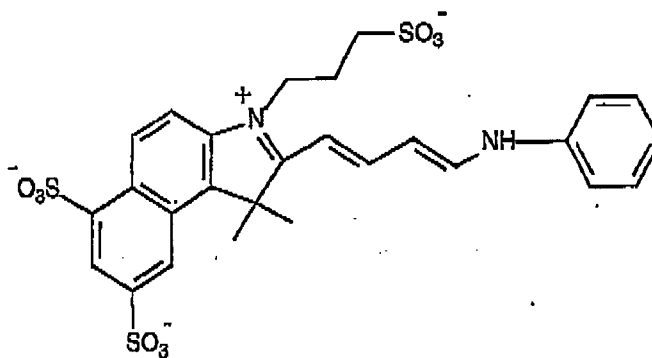
Compound 28
