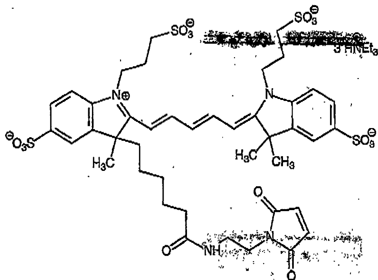
Compound 11
