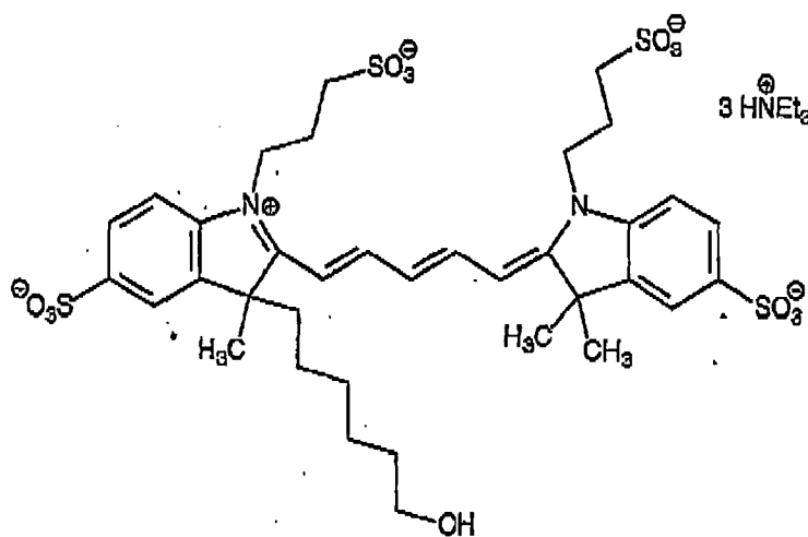
Compound 16
