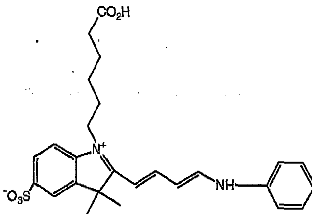
Compound 54
