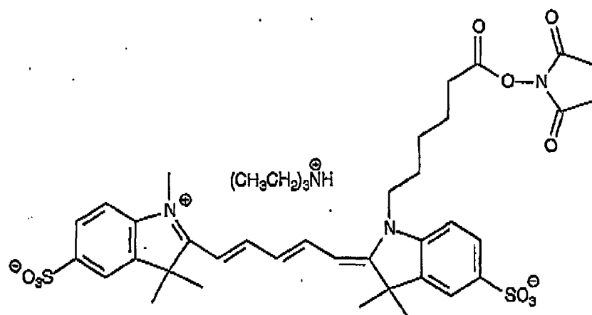
Compound 30
