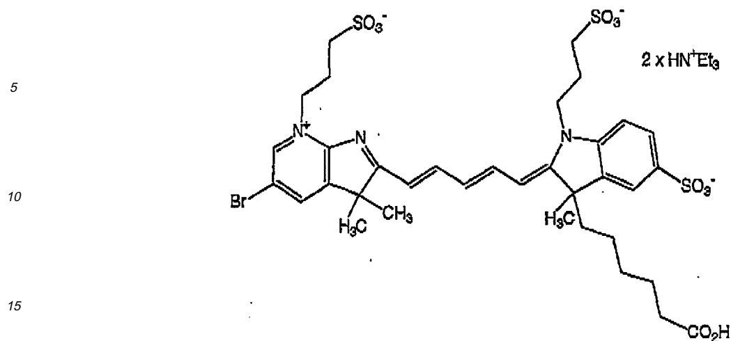
Compound 66
