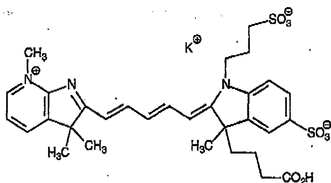
Compound 72
