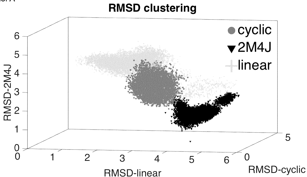
Fig. 9: RMSD-clustering plots
