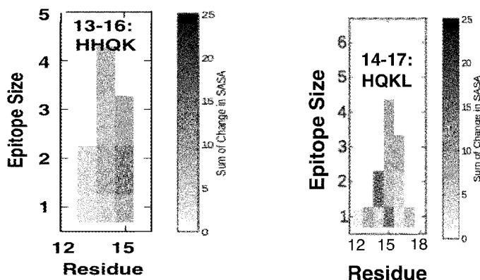
Fig. 1: Prediction using Collective Coordinate method and ProMis Go method Panel A: Collective Coordinates prediction (2MXU, left and for 2M4J, right)
