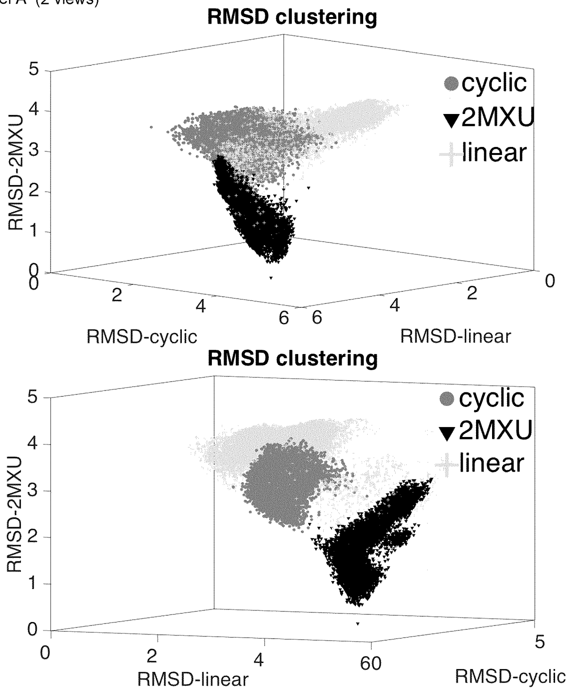
Fig. 10: RMSD-clustering plots for fibrils 2MXU, 2LMN and 2LMP
