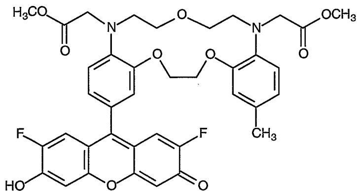
Compound 22
