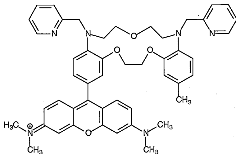
Compound 81
