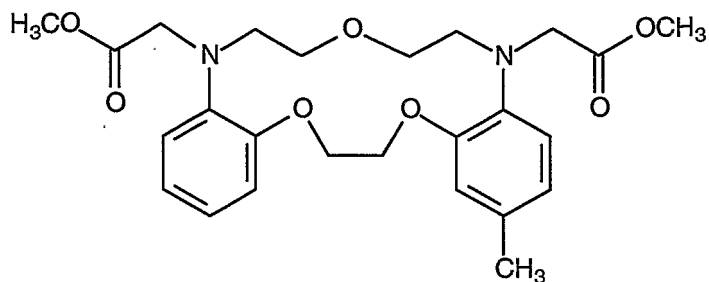
Compound 12
