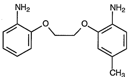
Compound 9
