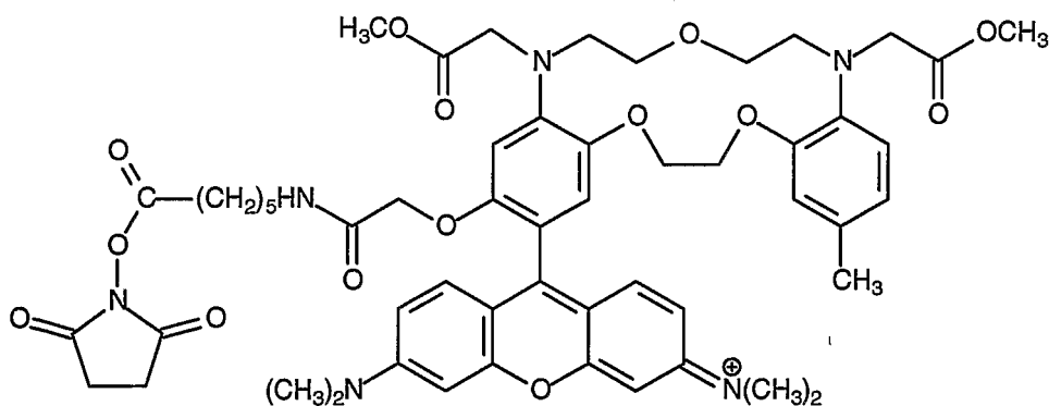
Compound 44
