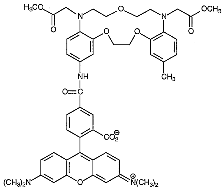
Compound 68
