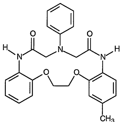
Compound 69
