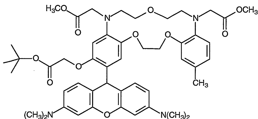
Compound 37
