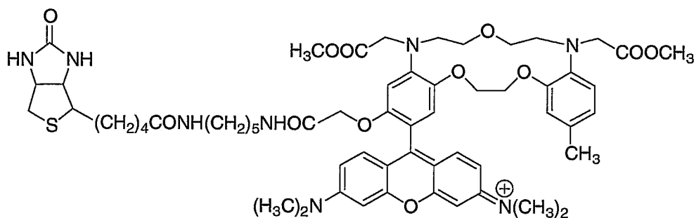
Compound 76
