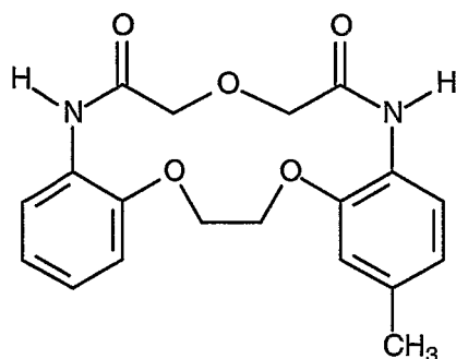
Compound 10
