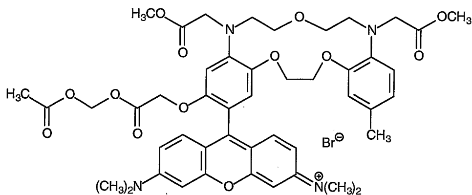
Compound 40
