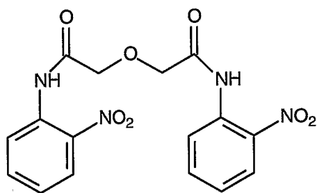
Compound 1
