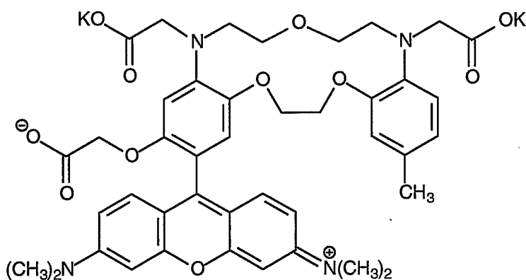
Compound 60
