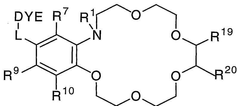
Formula (II)(d),
