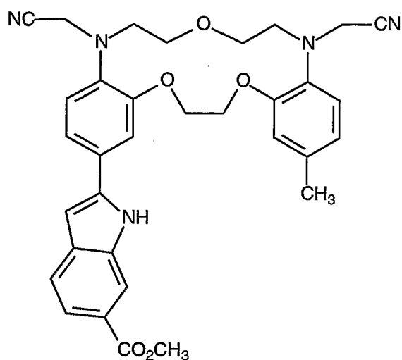
Compound 63
