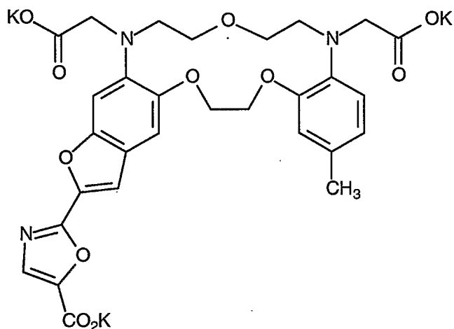
Compound 54
