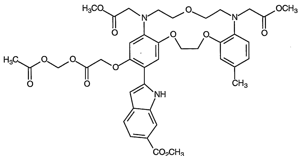
Compound 59
