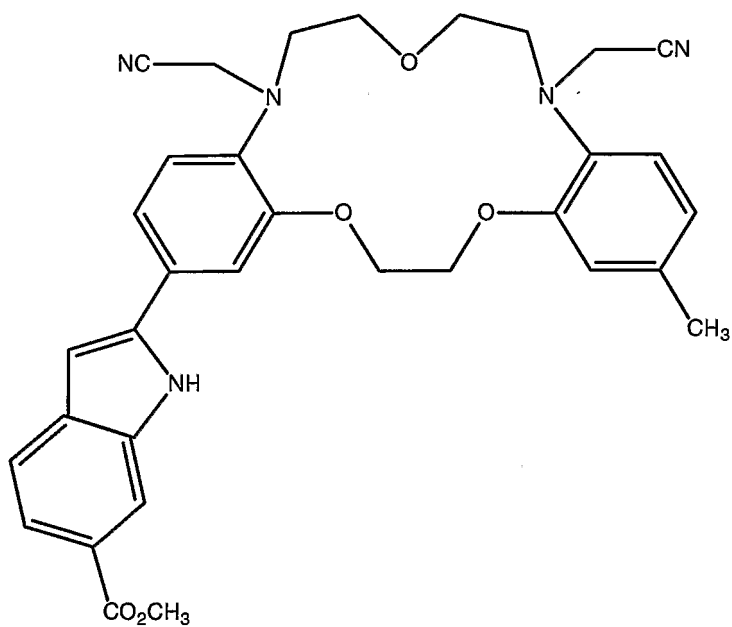
Compound 63
