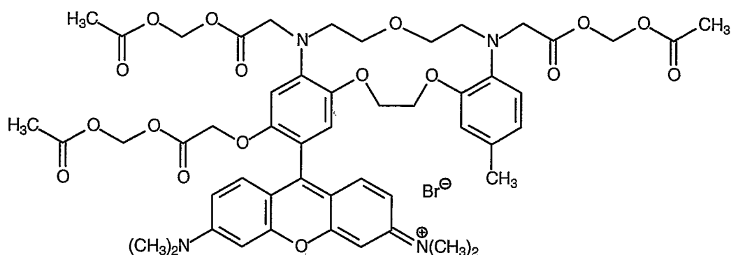
Compound 61
