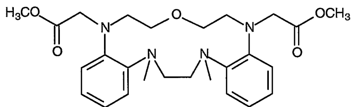
Compound 6
