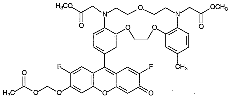
Compound 24
