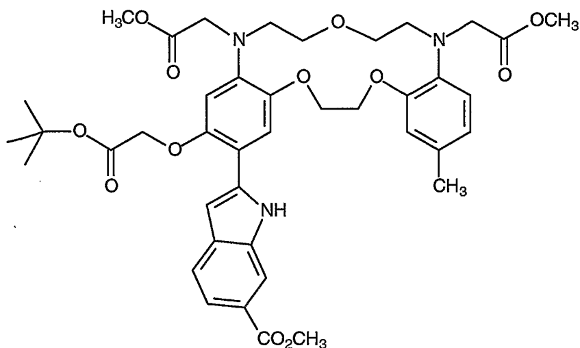
Compound 57
