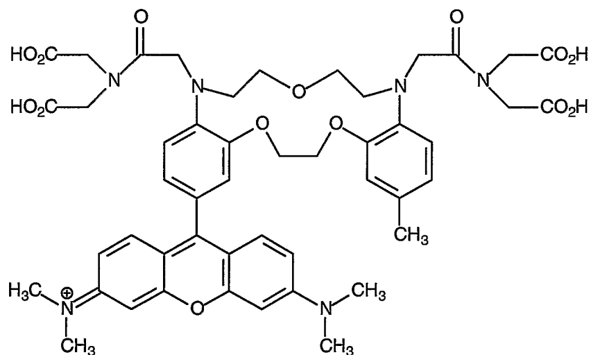
Compound 80
