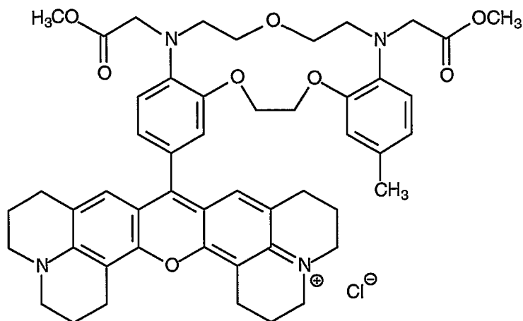
Compound 30
