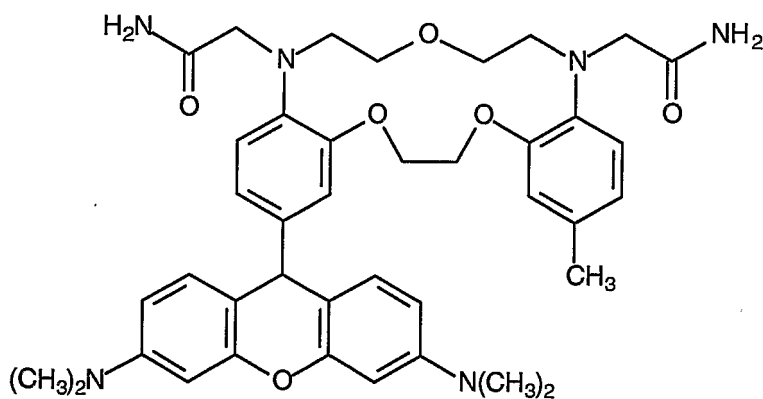
Compound 64
