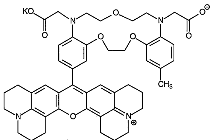
Compound 31
