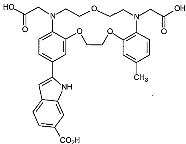
Compound 35
