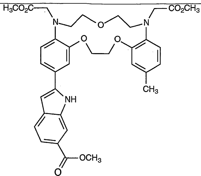
Compound 34
