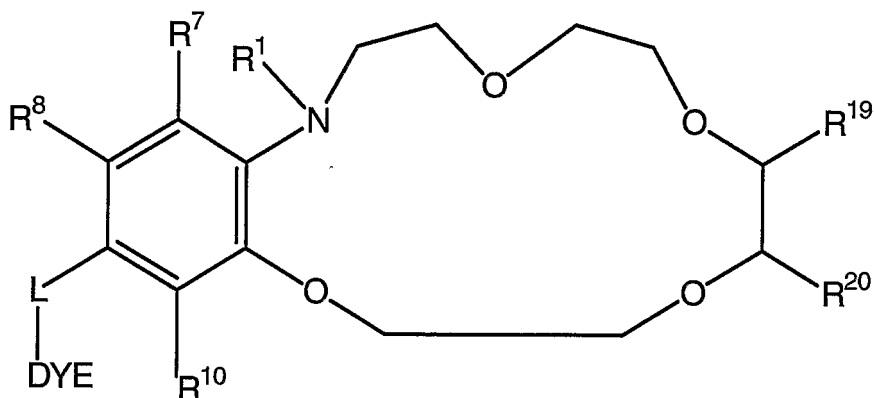
Formula (II)(a),
