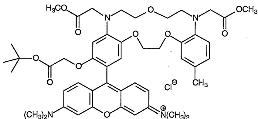
Compound 38
