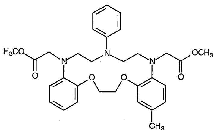
Compound 71
