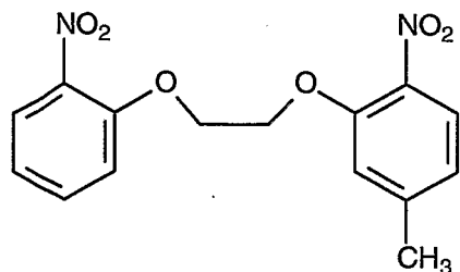
Compound 8
