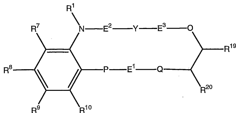
Formula (II)
