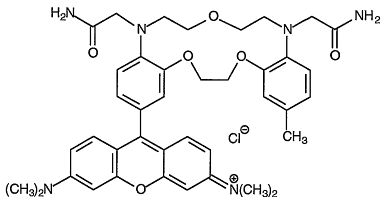
Compound 65
