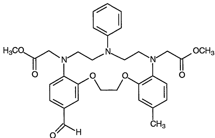
Compound 72
