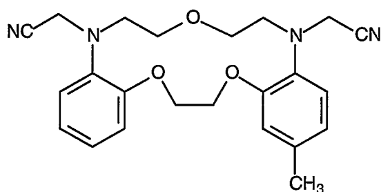
Compound 17
