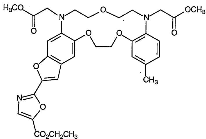
Compound 53
