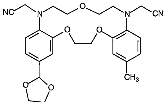
Compound 19
