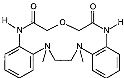
Compound 4
