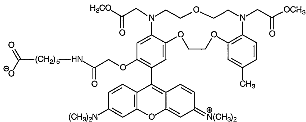
Compound 43
