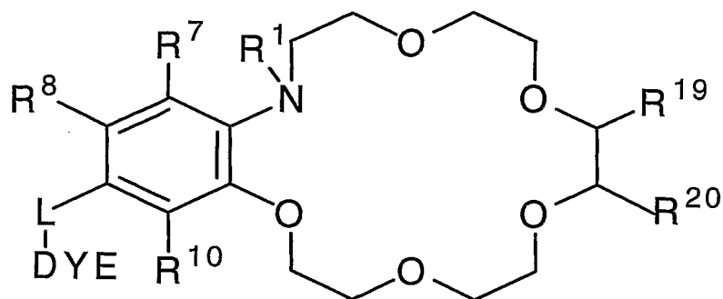
Formula (II)(c),
