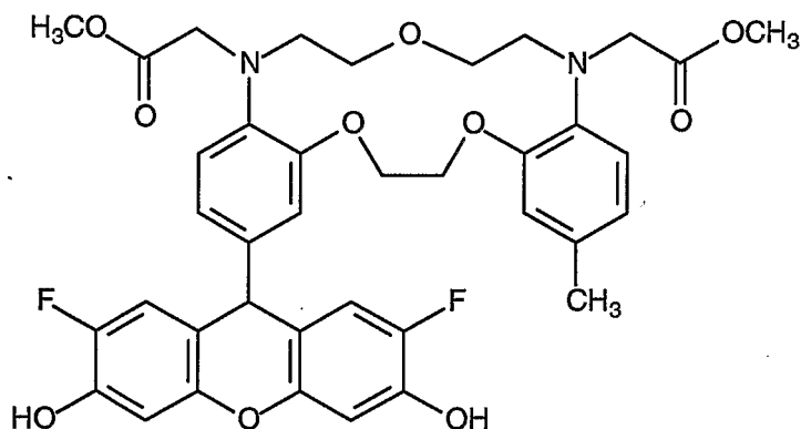
Compound 21
