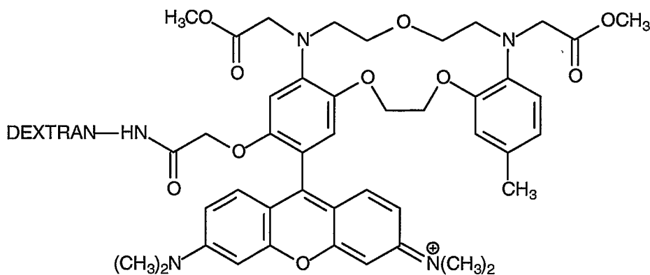
Compound 45
