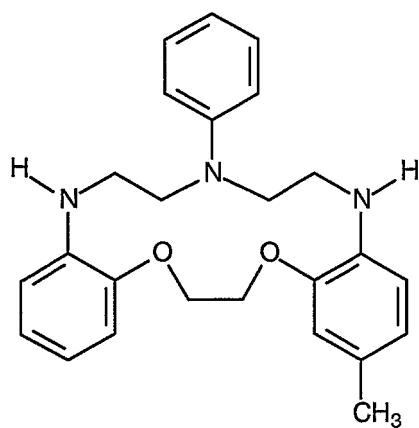
Compound 70
