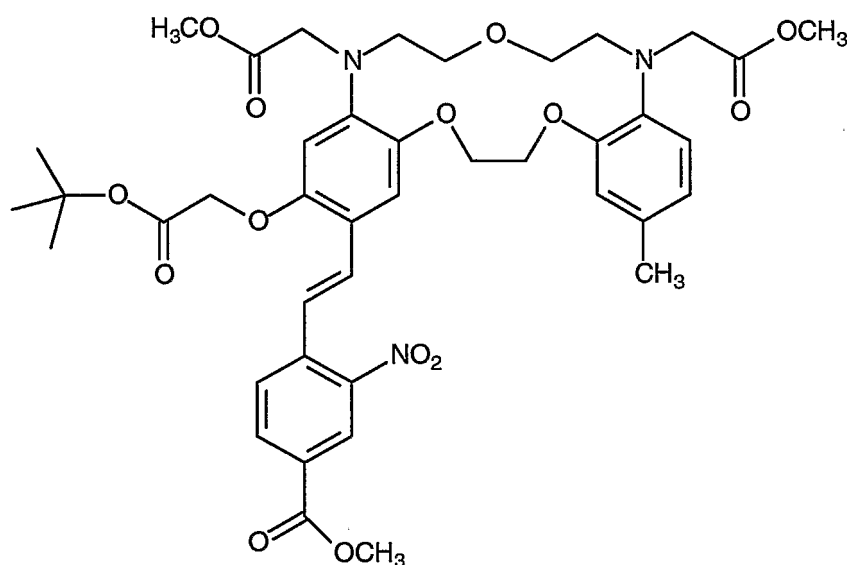
Compound 56
