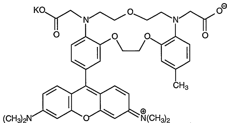
Compound 28
