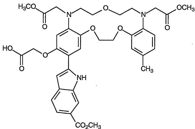
Compound 58
