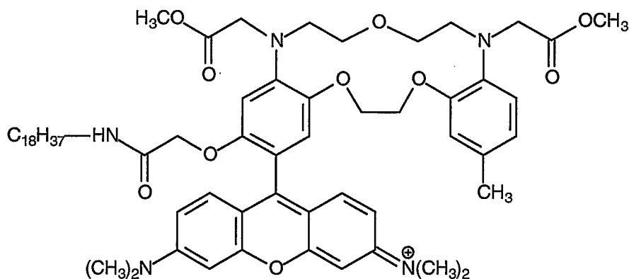
Compound 42
