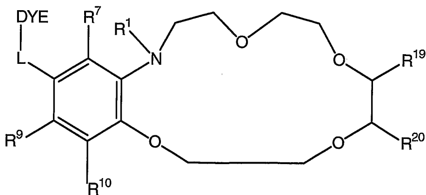
Formula (II)(b),
