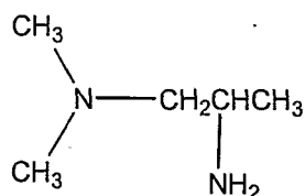
1-dimethylamino-2-propylamine
