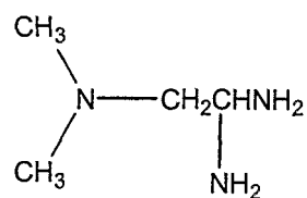
N,N-dimethylguanidine
