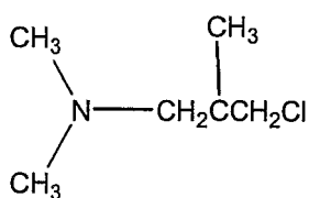
3-dimethylamino-2-methylpropyl chloride
