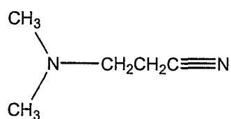
3-dimethylaminopropionitrile
