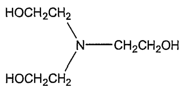
triethanolamine
