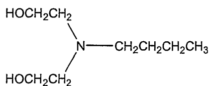
N-butyldiethanolamine
