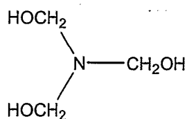
trimethanolamine
