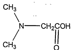
N,N-dimethylglycine
