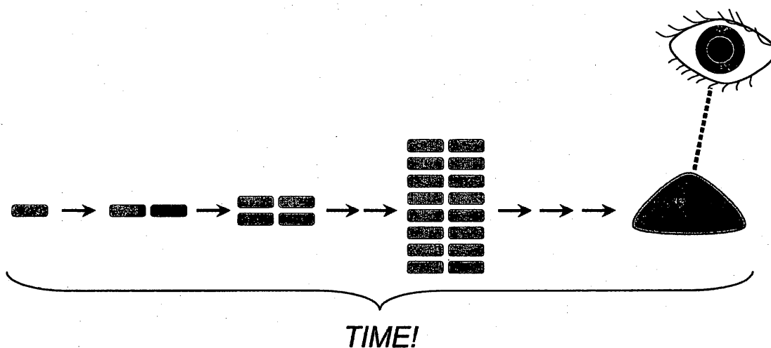
FIG. 1. Traditional microbial culture requires many generations of cell division
