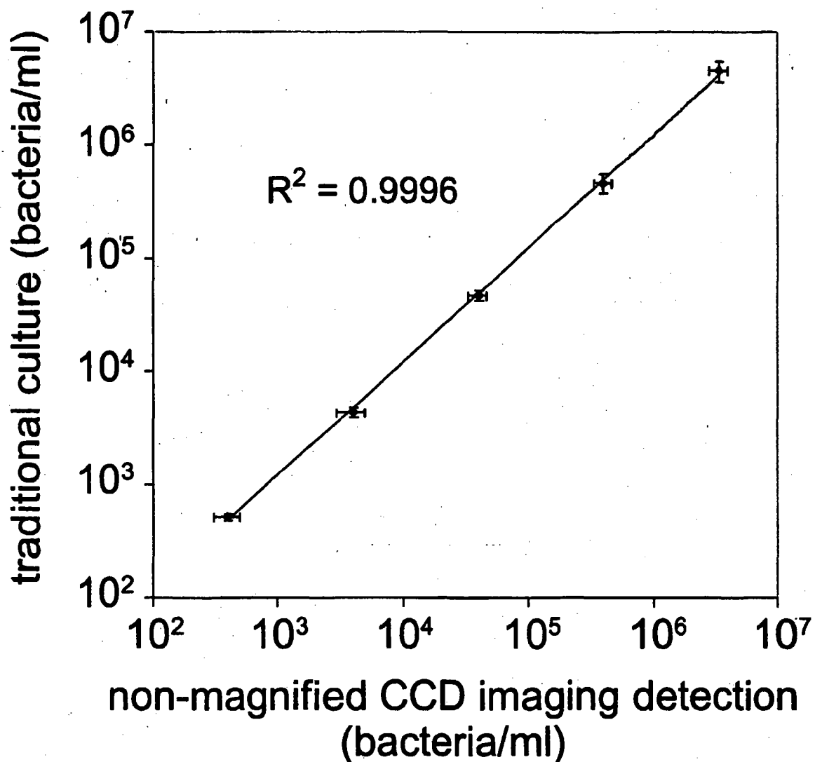
FIG. 12. Correlation between enumeration tests using the invention and traditional culture (Example 7).
