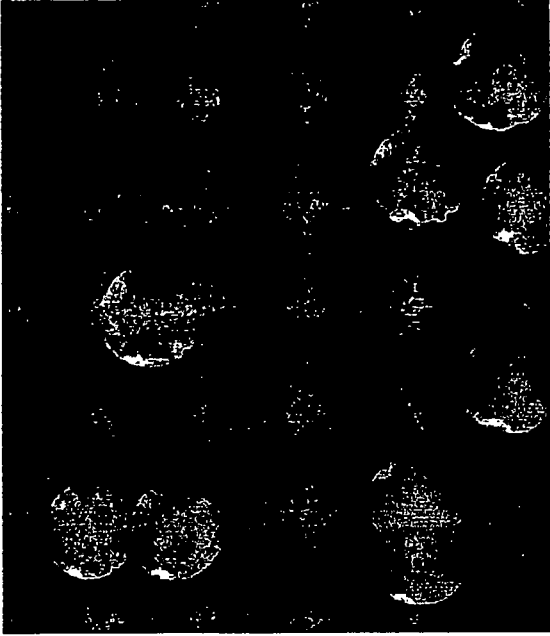
visible macrocolonies at 20 hr
