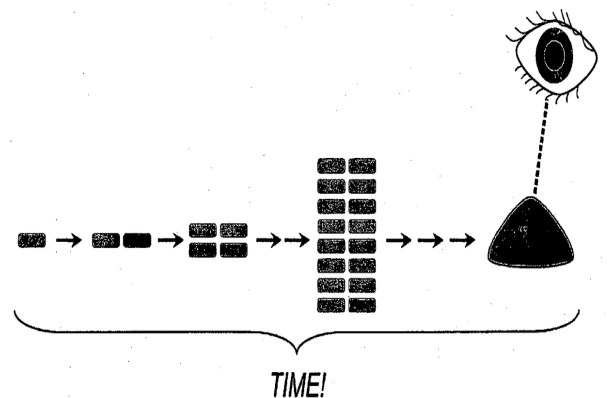
FIG. 1. Traditional microbial culture requires many generations of cell division
