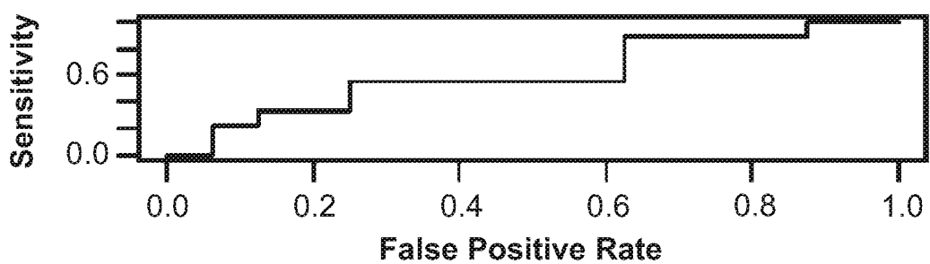
ROC Curve for PTX3; AUC= 0.611
