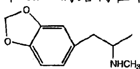
1 MDMA (Ecstasy)
