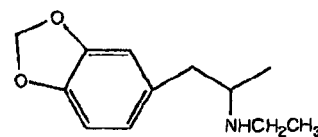
2 MDEA (Eve)
