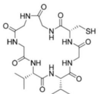
环状 (CGGGVVG)
