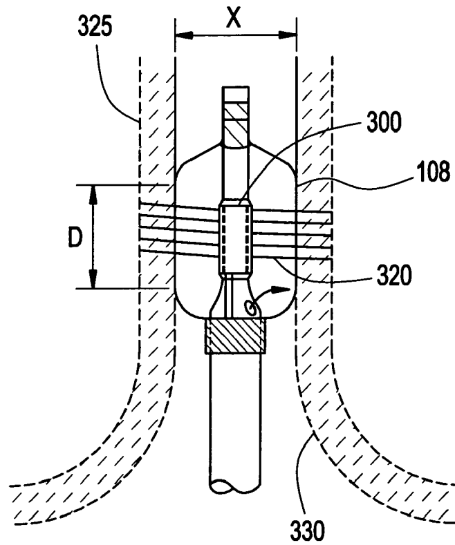
FIG. 3D PRIOR ART
