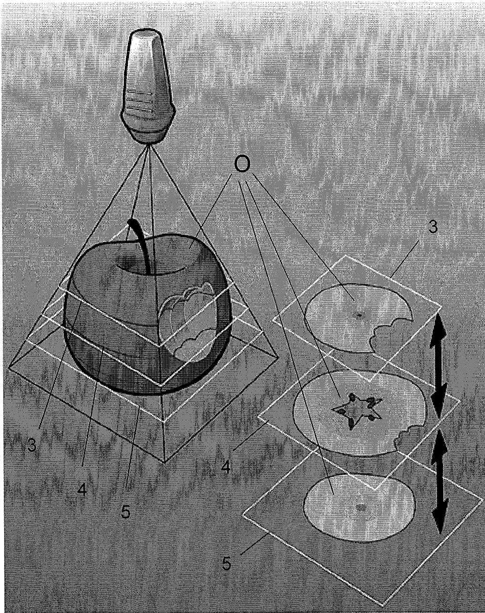
Figure 7. Sketch of cutting a three-dimensional dataset with transversal planes that are orthogonal to the principal planes like those employed in figure 6.
