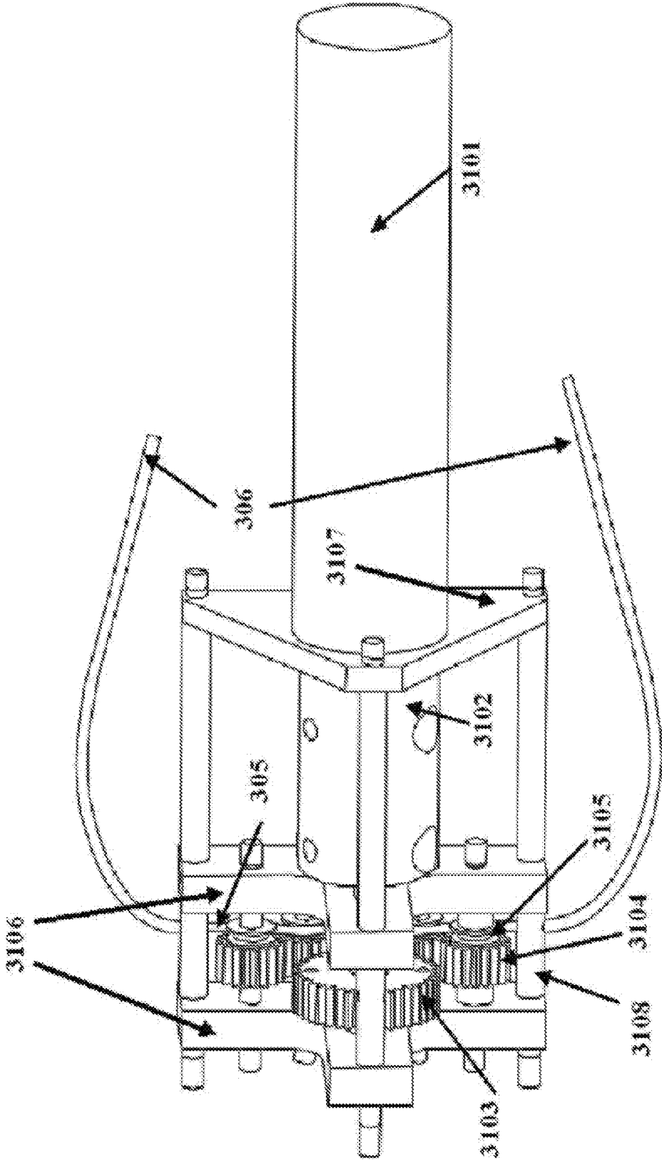
FIG.8A
