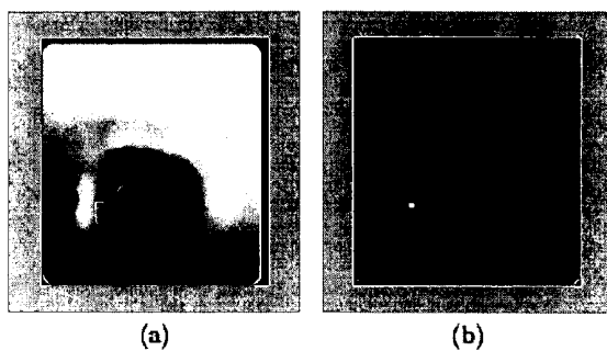
Figure 7. Illustration of the matching method used to compute the correspondence between a virtual and real image for the registration step in Section 2.4.1. (a) Virtual image with a black point to be matched in the real image on right. (b) Real image with the white point showing the initial guess for the match and the black point showing the final match.
