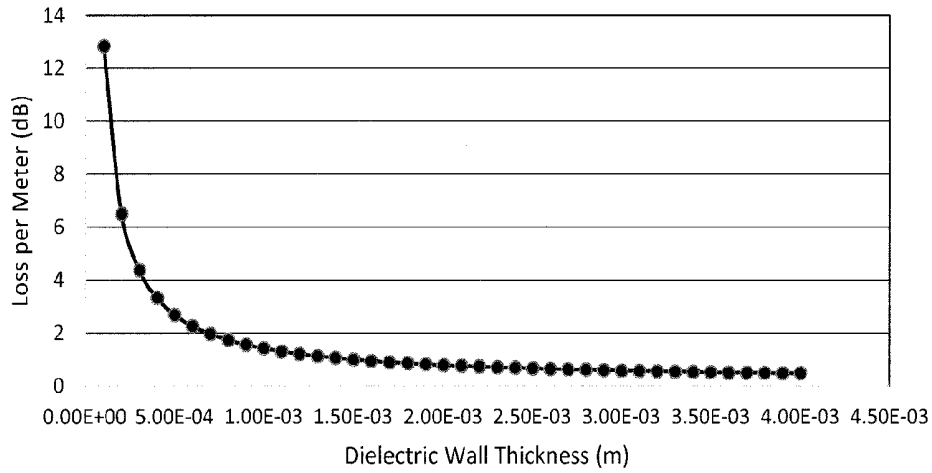
Loss per metre of integrated energy conveying structure
