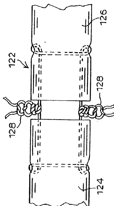
PRIOR ART FIG. 24
