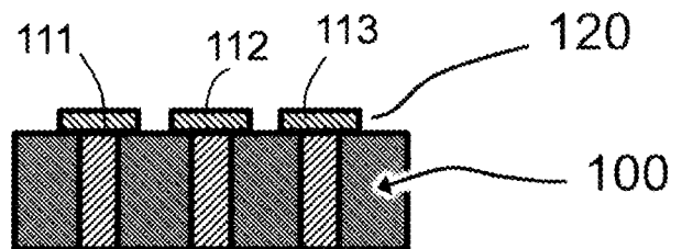
Section G-G
