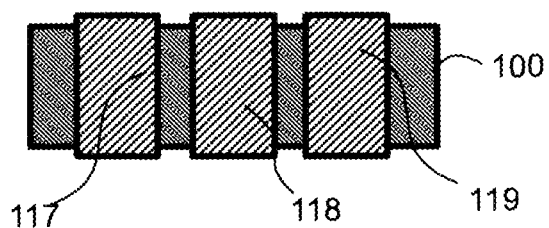
Section DD-DD
