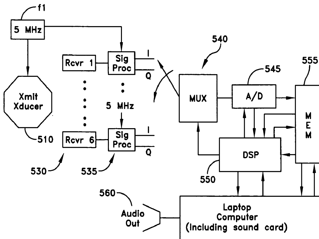
Carotid Screening System with Synthetic Doppler Audio
