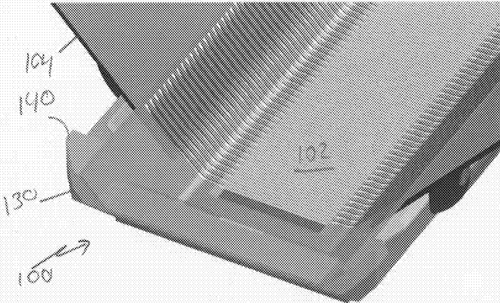
Figure 13: Close up view of Electrodes showing insulation of signal electrodes from ground path through conductive support structure
