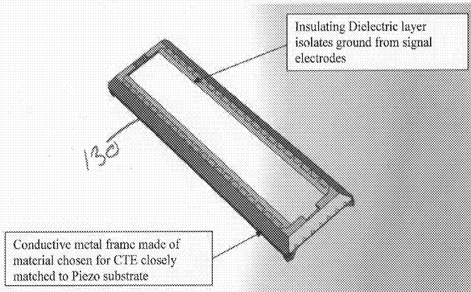
Figure 3: Conductive hybrid tapered support structure - bottom view.
