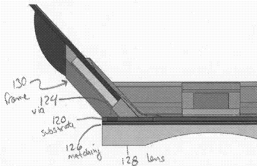
Figure 15: Close up of one side of cross section view of electrically complete array transducer with lens and matching layers, showing ground path with via, and signal electrode with insulating layer of hybrid support structure in place.
