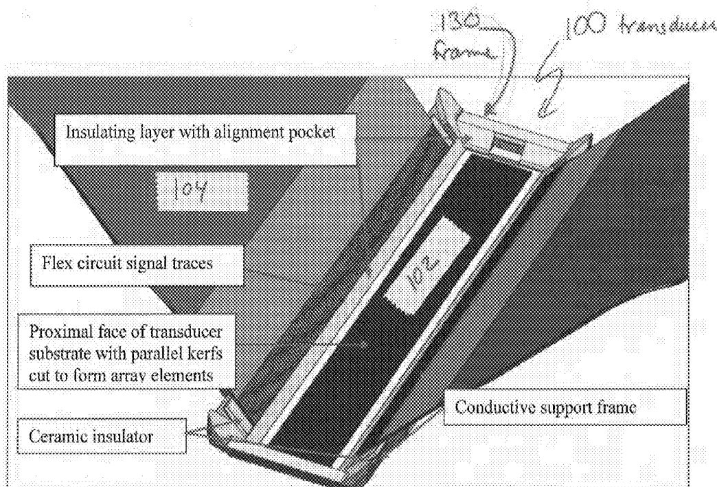
Flexible PCBs bonded to a ceramic insulator in turn bonded into a pocket formed in the insulating upper portion of a conductive support structure (hybrid tapered support).
