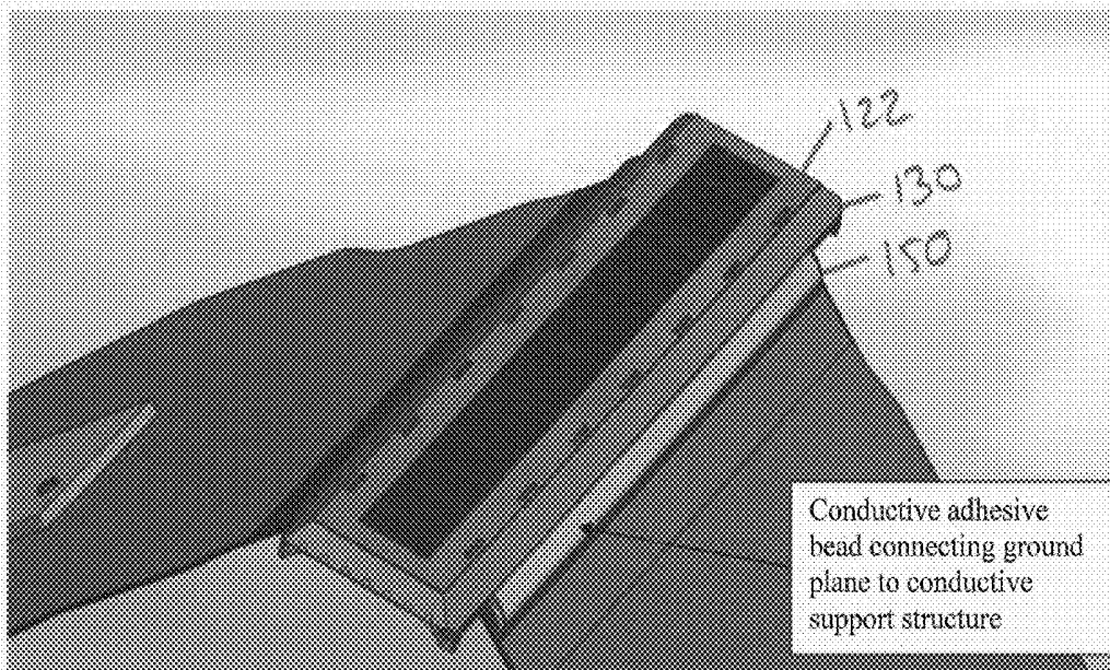
Figure 9: Conductive adhesive used to connect the copper ground plane of the PCB to the conductive support structure
