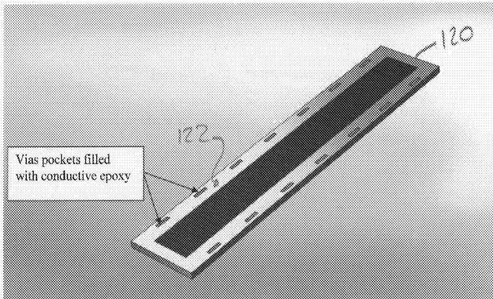
Figure 6: Via pockets filled with conductive epoxy viewed from ground plane side
