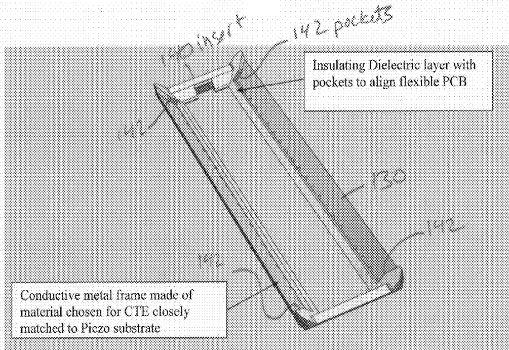
Figure 2: Conductive hybrid tapered support structure - top view
