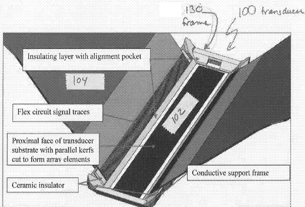
Figure 1: Flexible PCBs bonded to a ceramic insulator in turn bonded into a pocket formed in the insulating upper portion of a conductive support structure (hybrid tapered support).
