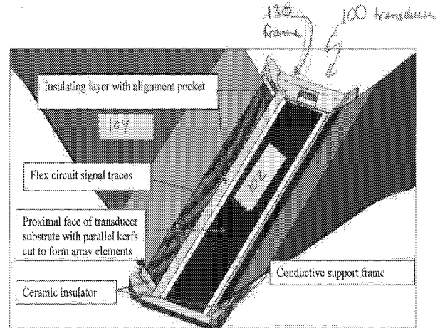
Flexible PCBs bonded to a ceramic insulator in turn bonded into a pocket formed in the insulating upper portion of a conductive support structure (hybrid tapered support).
