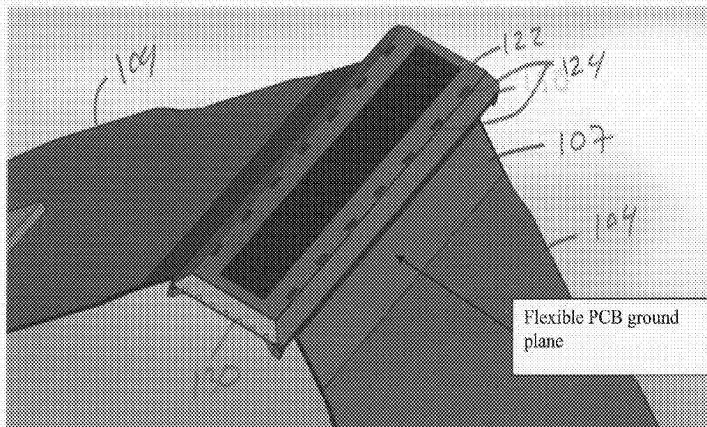
Figure 8: Assembled array transducer with flexible PCBs attached. No electrical connection to ground plane.
