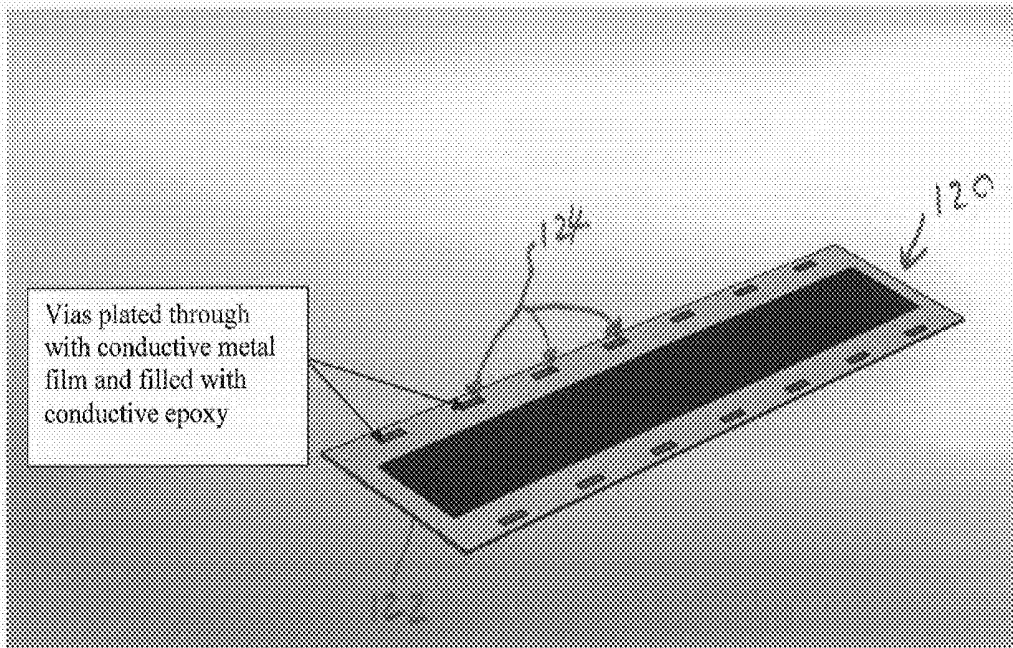
Figure 7: Completed vias viewed from inner (signal electrode) side of transducer substrate after thinning the transducer substrate to the final dimension.
