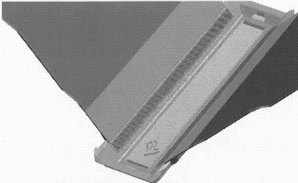
Figure 12: Complete signal electrode pattern in place on array transducer
