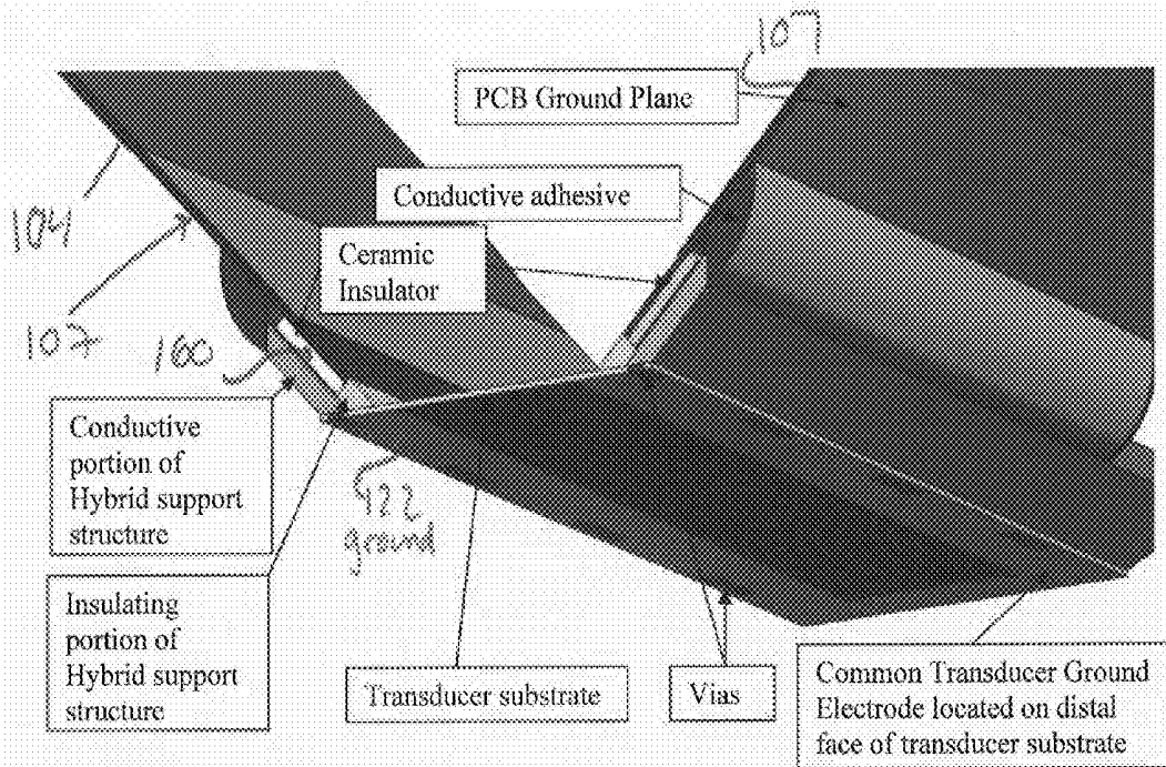
Figure 10: Cross section oblique view showing the vias making connection from the outside facing ground plane to the conductive support structure, then through conductive adhesive and finally to the ground plane of the flexible PCB.
