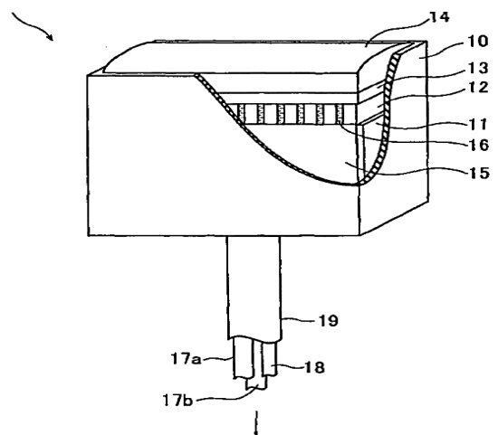
TO ULTRASONIC DIAGNOSTIC APPARATUS MAIN BODY
