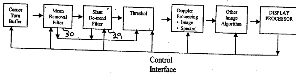
Figure 5: Alternative Ultrasound Data Flow
