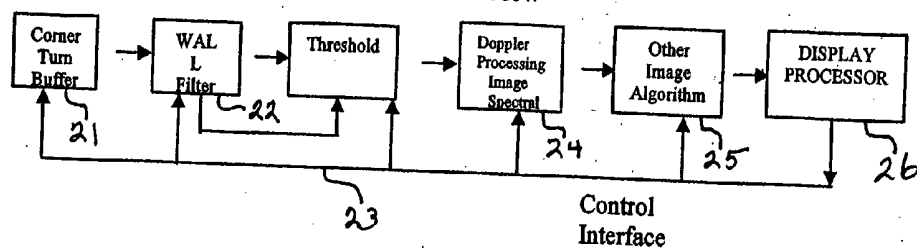
Figure 3: Ultrasound Data Flow
