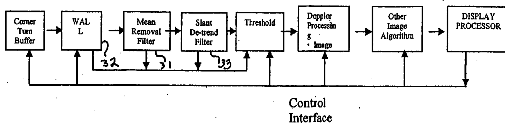
Figure 6: Improved Cascaded Filtered Ultrasound Data Flow
