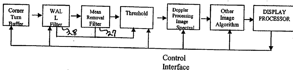
Figure 4: Modified Ultra Sound Data Flow
