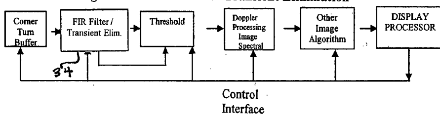
Figure 7: FIR Filter with Transient Elimination
