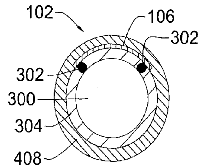
Section 2-2
