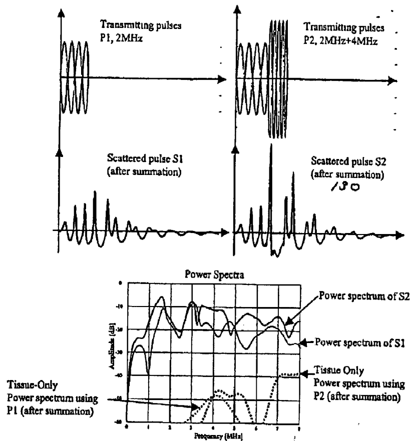
Simulated enhancement of the pulse inversion imaging using a pair of phase-inverted stepped-chirps (P2) compared with regular phase-inverted pulses (P1). Tissue responses are also simulated under these two situations.
