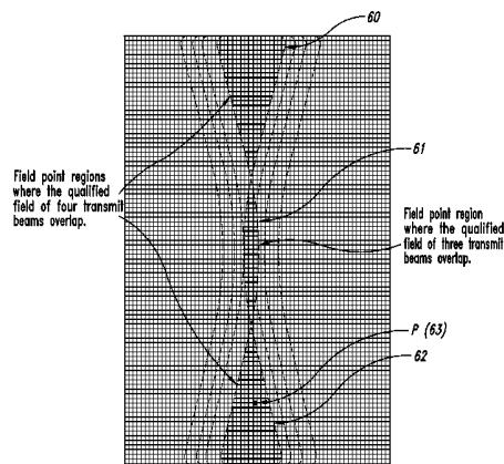
Four overlapping transmit beams, showing field points in overlapped regions where three or four received echo signals can be combined for image formation.
