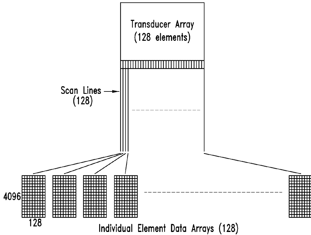
SCAN SEQUENCE AND DATA FOR A 128 ELEMENT LINEAR ARRAY
