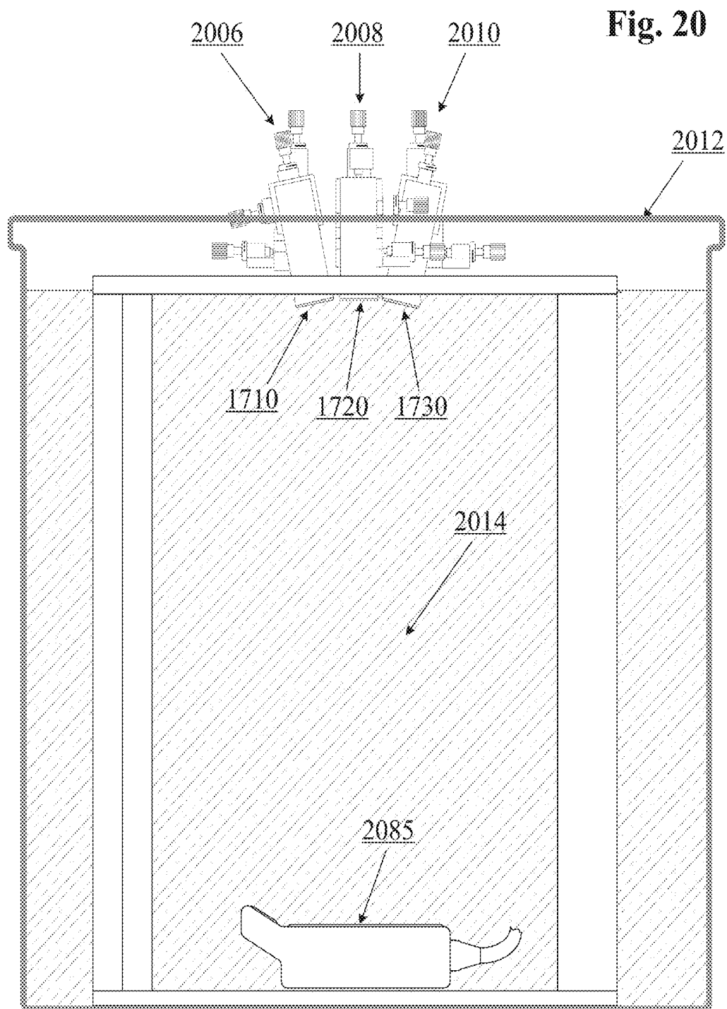
Assembled test fixture in tank.
