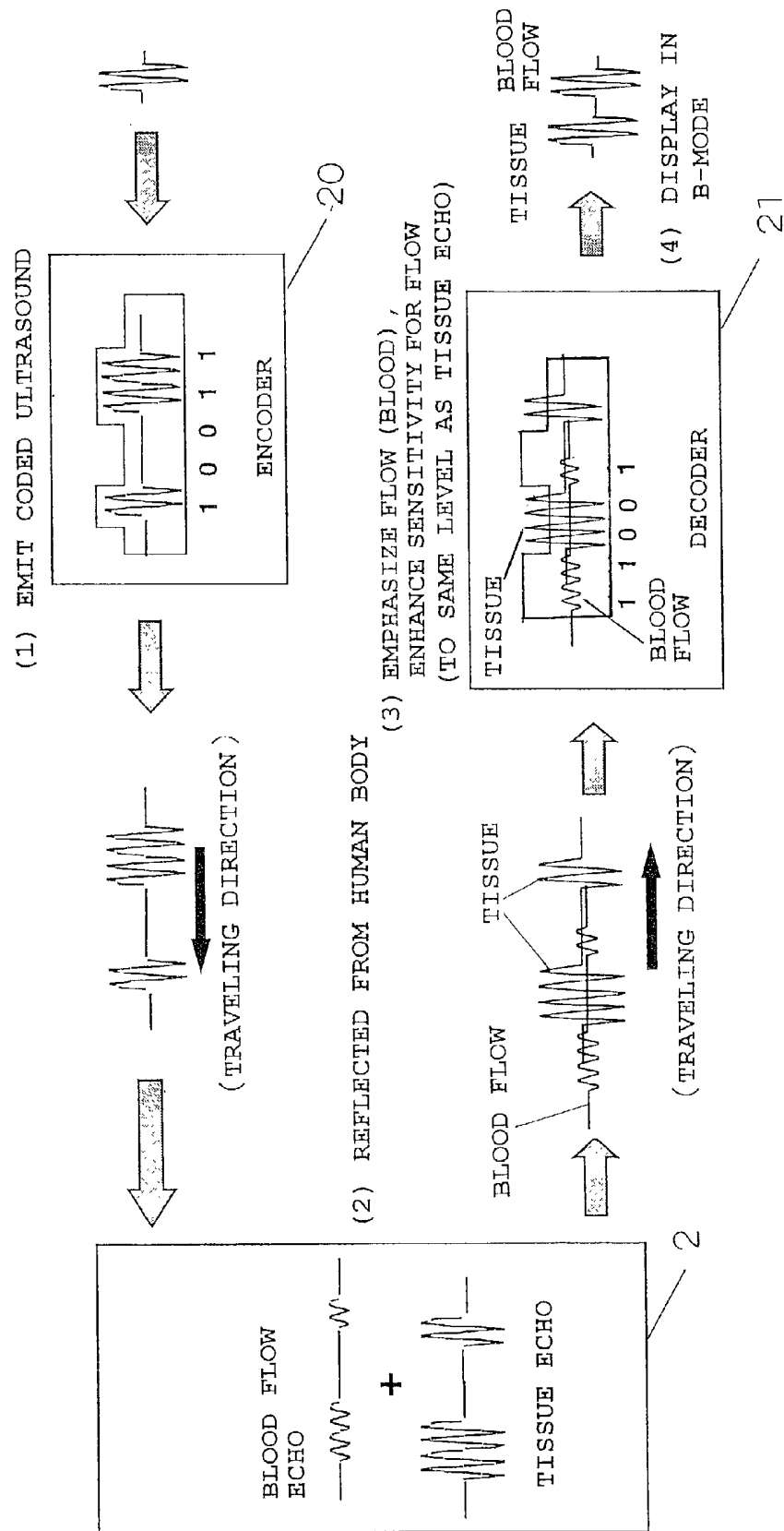
Fig. 10 PRIOR ART
