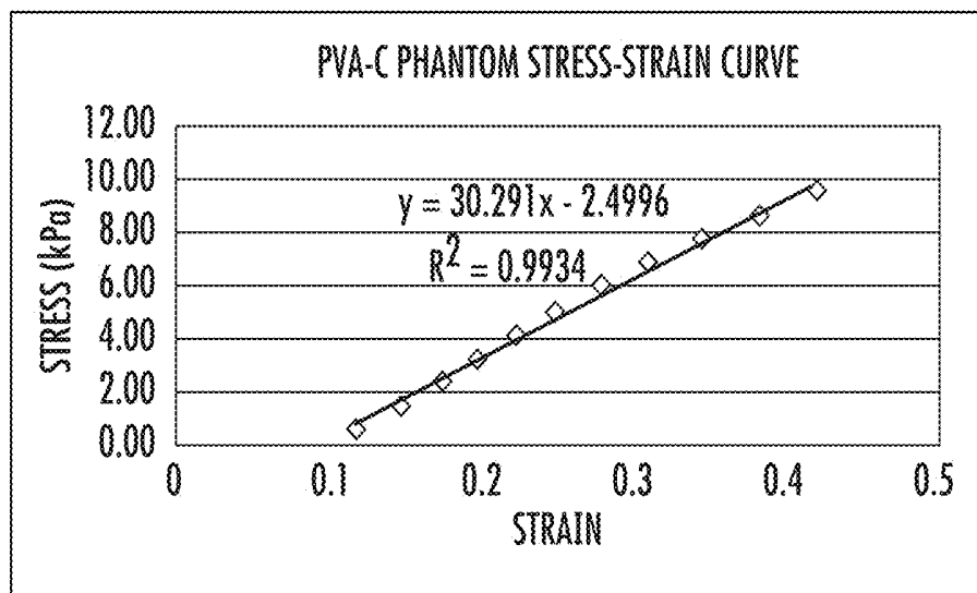
STRESS-STRAIN CURVE TO DETERMINE THE YOUNG'S MODULUS FOR PVA-C PHANTOM
