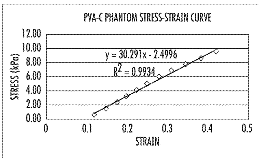
FIGURE 1. STRESS-STRAIN CURVE TO DETERMINE THE YOUNG'S MODULUS FOR PVA-C PHANTOM
