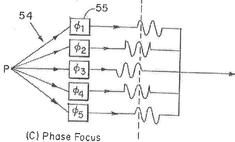
FIG. 2C Prior Art
